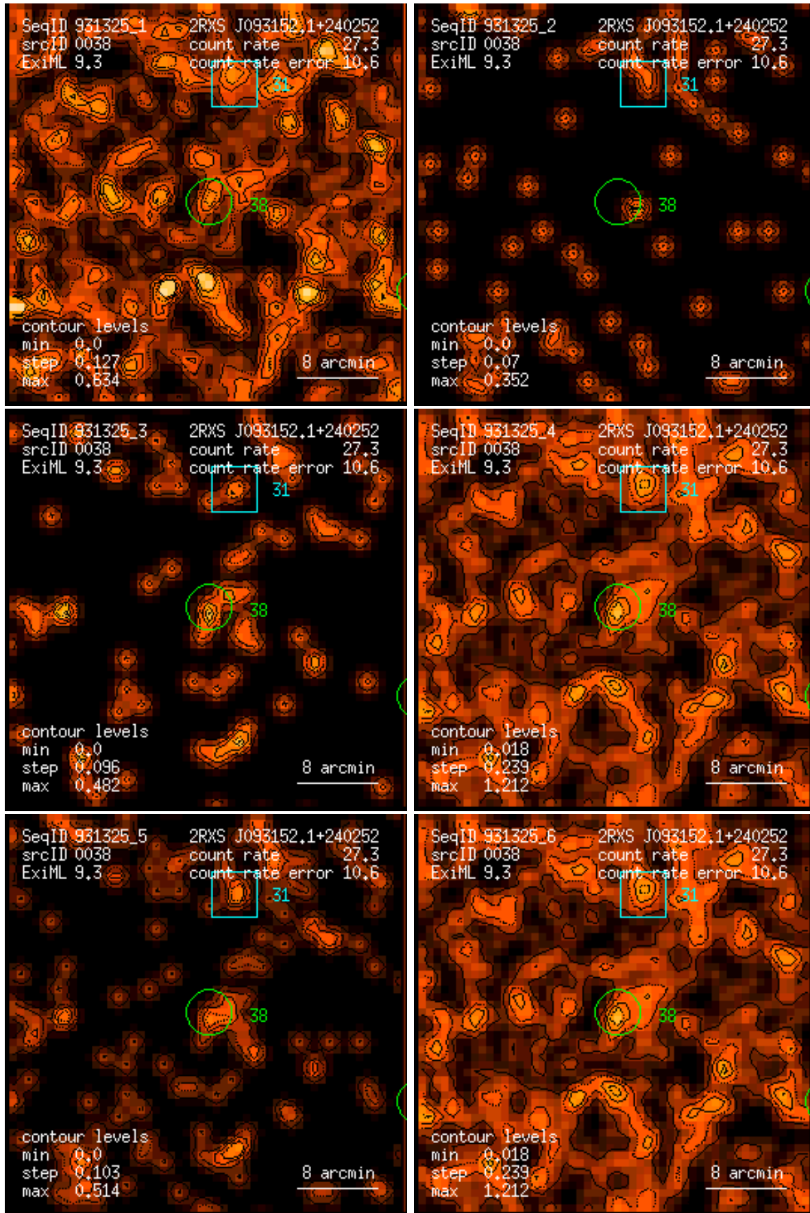
Figure 38: RASS 931325: detection 0038: band rate images, Gaussian filter: (1) PSPC channels 11 – 41, (2) 52 – 90, (3) 91 – 201, (4) 11 – 235, (5) 52 – 201, (6) 11 – 201. Broad band rates in counts/ks. Band rate contour levels in counts/ks/arcmin 2 .
