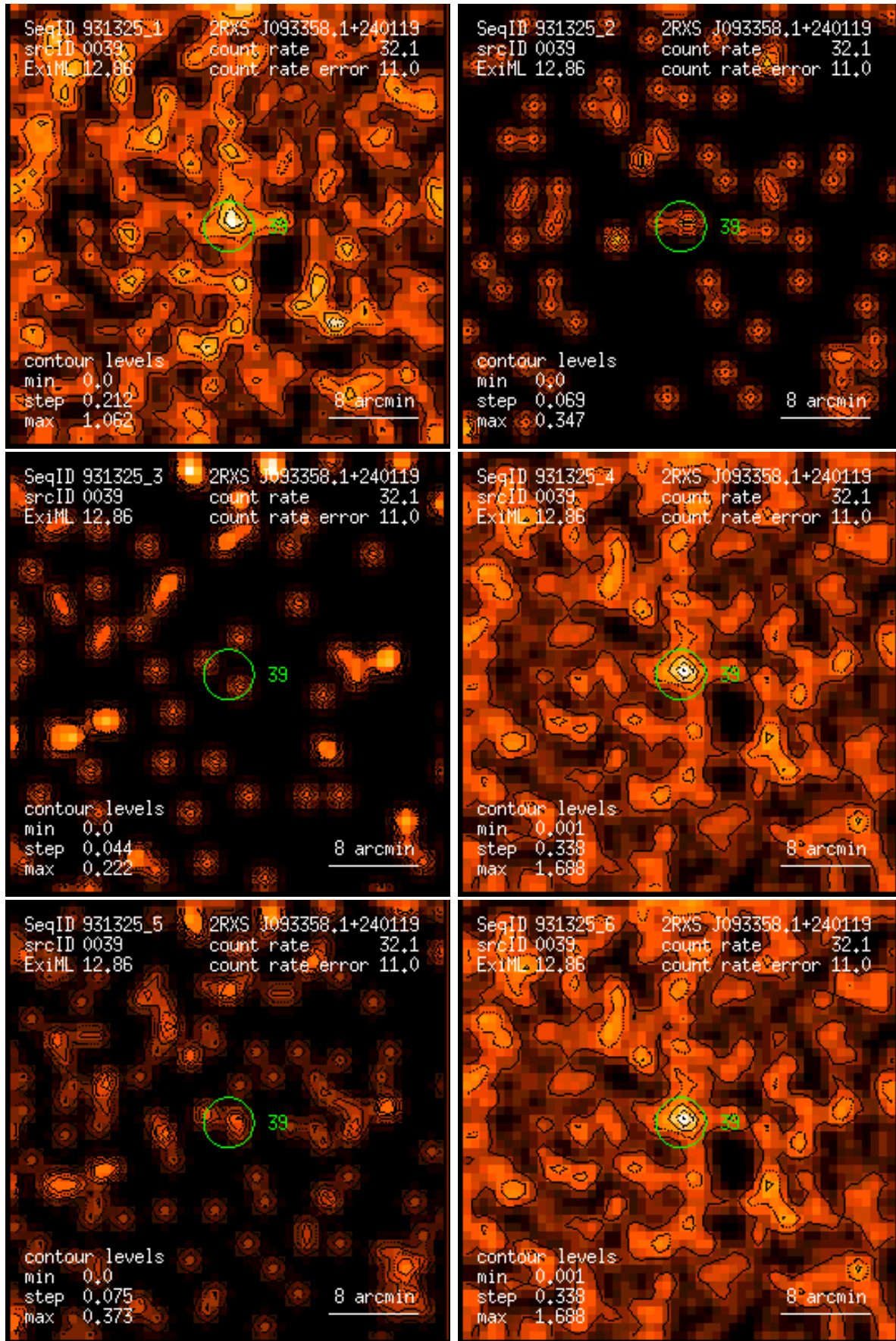
Figure 39: RASS 931325: detection 0039: band rate images, Gaussian filter: (1) PSPC channels 11 – 41, (2) 52 – 90, (3) 91 – 201, (4) 11 – 235, (5) 52 – 201, (6) 11 – 201. Broad band rates in counts/ks. Band rate contour levels in counts/ks/arcmin 2 .
