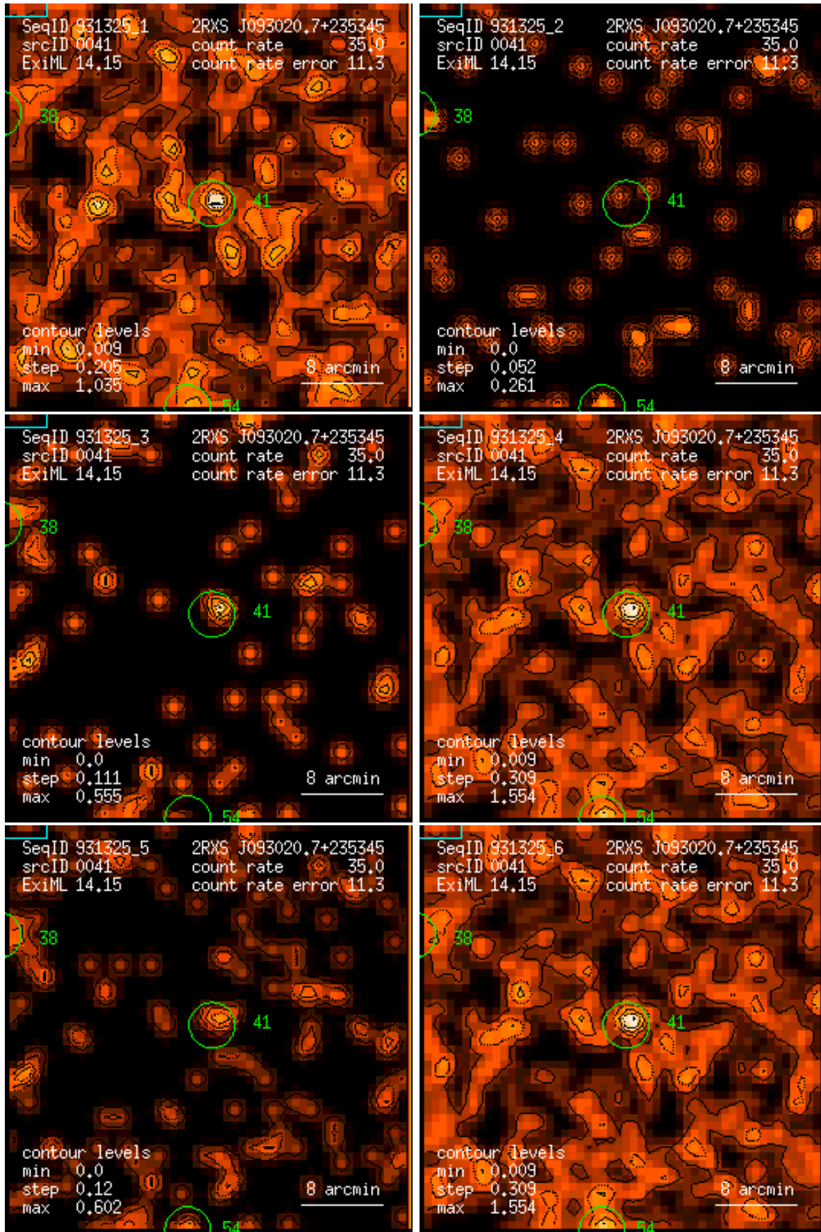
Figure 41: RASS 931325: detection 0041: band rate images, Gaussian filter: (1) PSPC channels 11 – 41, (2) 52 – 90, (3) 91 – 201, (4) 11 – 235, (5) 52 – 201, (6) 11 – 201. Broad band rates in counts/ks. Band rate contour levels in counts/ks/arcmin 2 .
