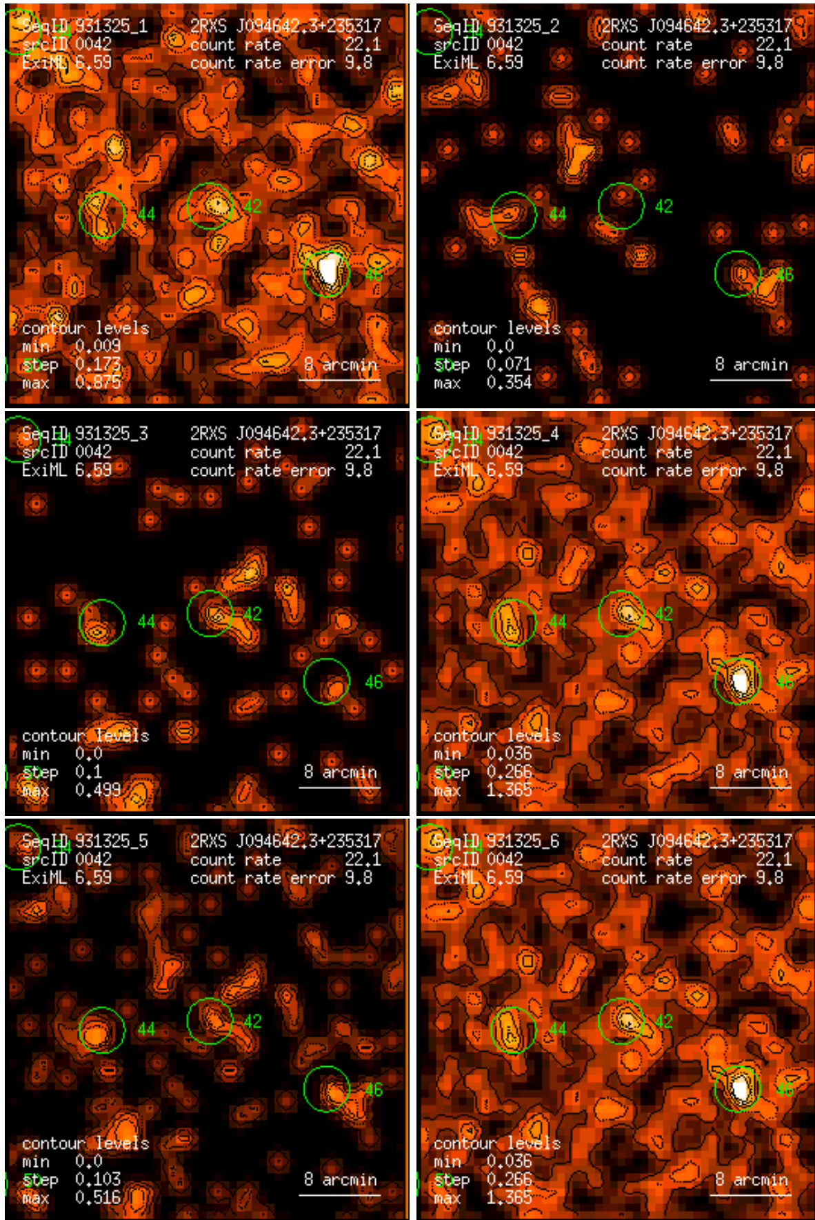
Figure 42: RASS 931325: detection 0042: band rate images, Gaussian filter: (1) PSPC channels 11 – 41, (2) 52 – 90, (3) 91 – 201, (4) 11 – 235, (5) 52 – 201, (6) 11 – 201. Broad band rates in counts/ks. Band rate contour levels in counts/ks/arcmin 2 .
