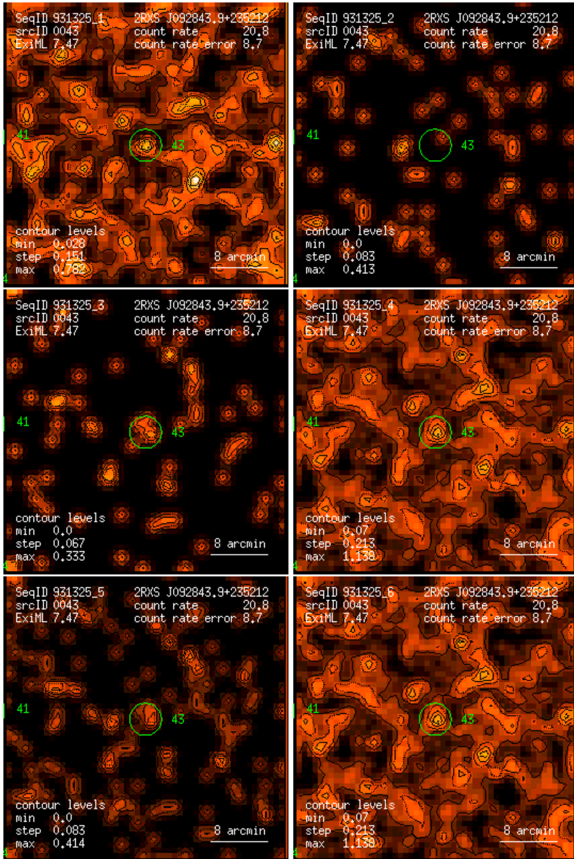
Figure 43: RASS 931325: detection 0043: band rate images, Gaussian filter: (1) PSPC channels 11 – 41, (2) 52 – 90, (3) 91 – 201, (4) 11 – 235, (5) 52 – 201, (6) 11 – 201. Broad band rates in counts/ks. Band rate contour levels in counts/ks/arcmin 2 .
