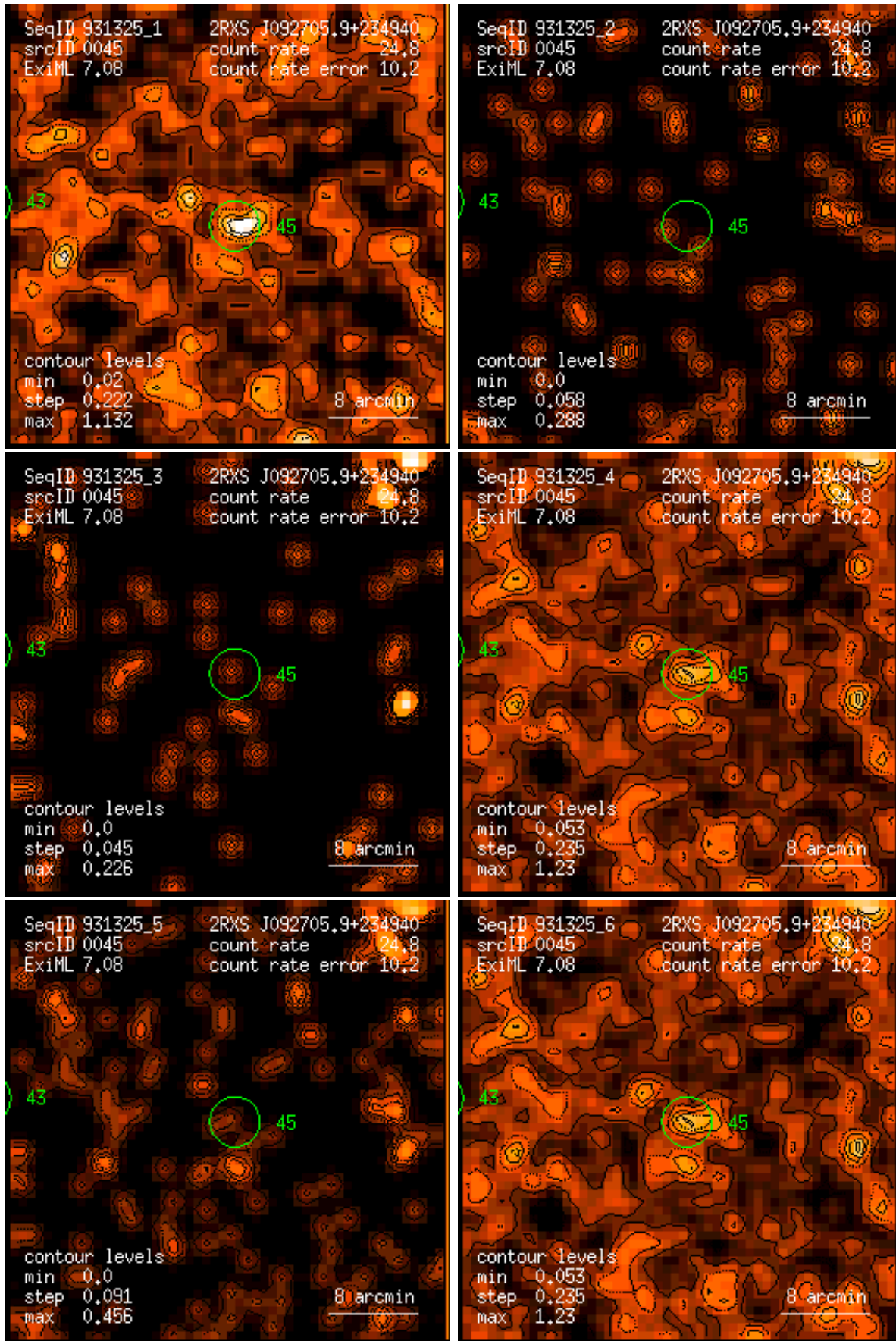
Figure 45: RASS 931325: detection 0045: band rate images, Gaussian filter: (1) PSPC channels 11 – 41, (2) 52 – 90, (3) 91 – 201, (4) 11 – 235, (5) 52 – 201, (6) 11 – 201. Broad band rates in counts/ks. Band rate contour levels in counts/ks/arcmin 2 .
