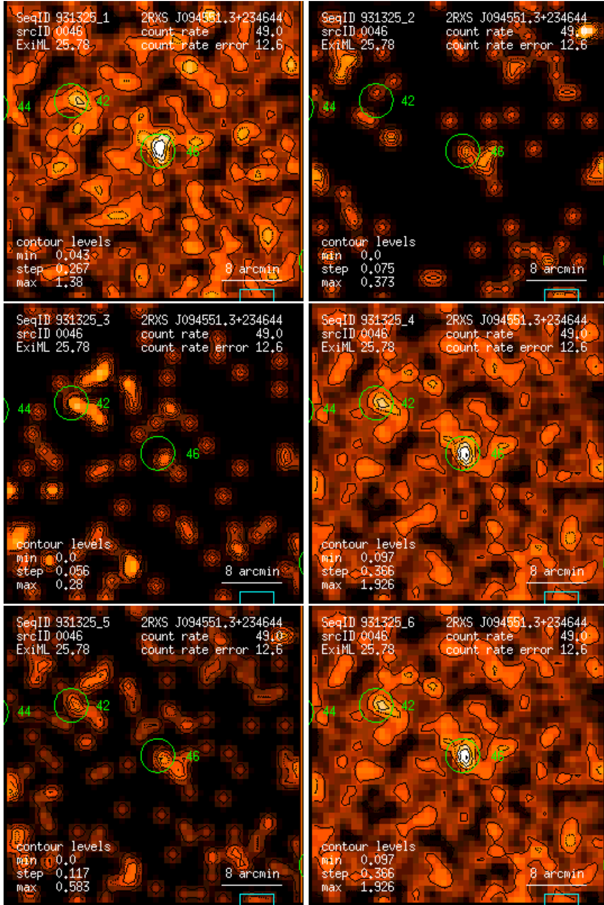
Figure 46: RASS 931325: detection 0046: band rate images, Gaussian filter: (1) PSPC channels 11 – 41, (2) 52 – 90, (3) 91 – 201, (4) 11 – 235, (5) 52 – 201, (6) 11 – 201. Broad band rates in counts/ks. Band rate contour levels in counts/ks/arcmin 2 .
