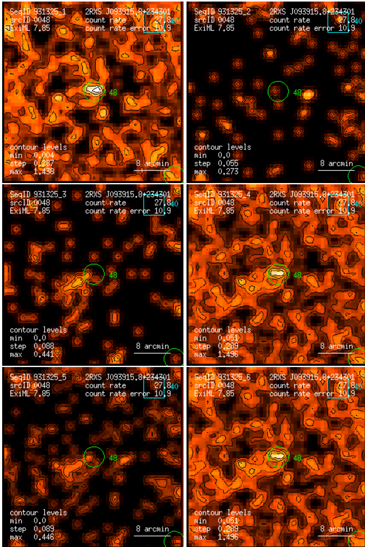
Figure 48: RASS 931325: detection 0048: band rate images, Gaussian filter: (1) PSPC channels 11 – 41, (2) 52 – 90, (3) 91 – 201, (4) 11 – 235, (5) 52 – 201, (6) 11 – 201. Broad band rates in counts/ks. Band rate contour levels in counts/ks/arcmin 2 .
