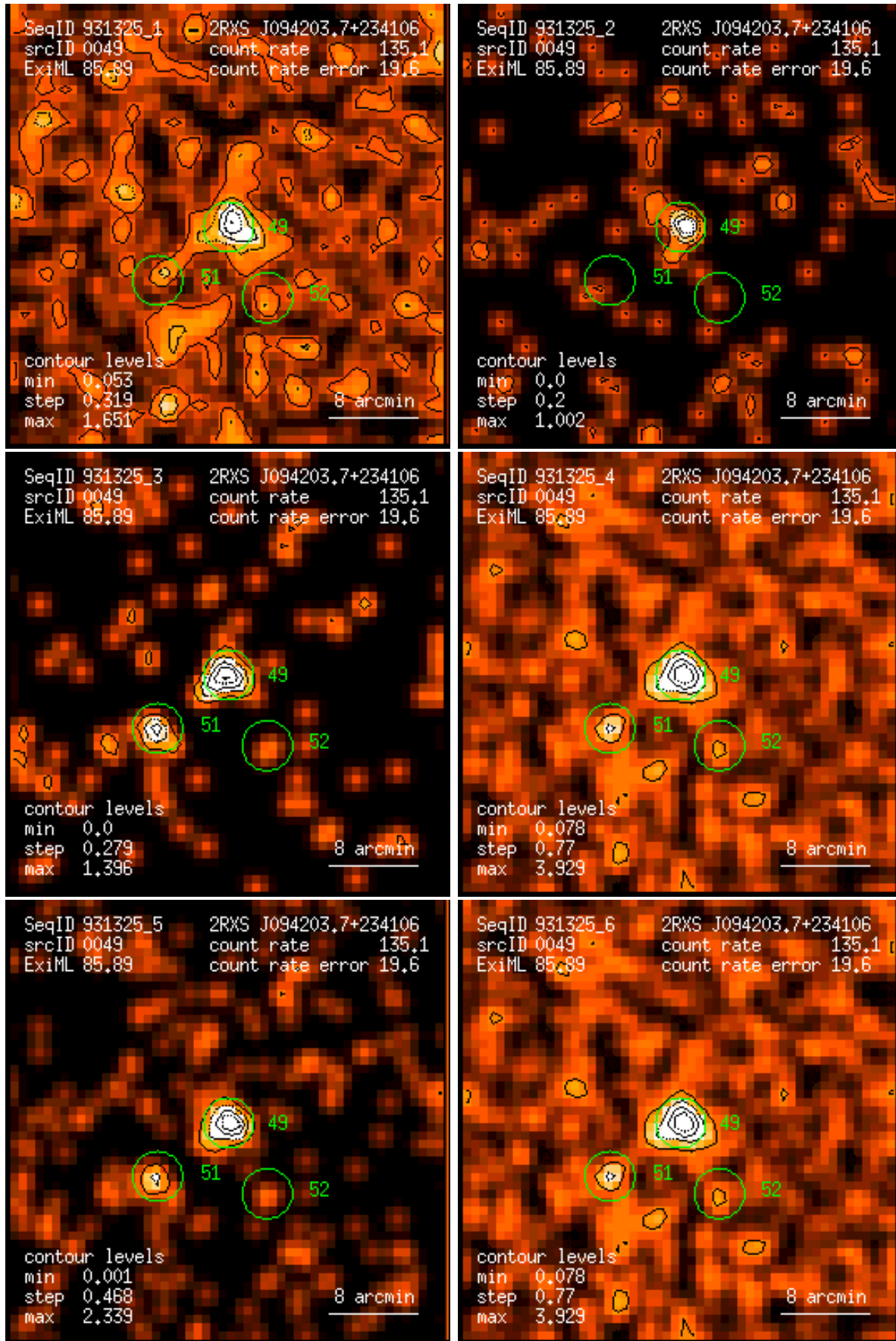
Figure 49: RASS 931325: detection 0049: band rate images, Gaussian filter: (1) PSPC channels 11 – 41, (2) 52 – 90, (3) 91 – 201, (4) 11 – 235, (5) 52 – 201, (6) 11 – 201. Broad band rates in counts/ks. Band rate contour levels in counts/ks/arcmin 2 .
