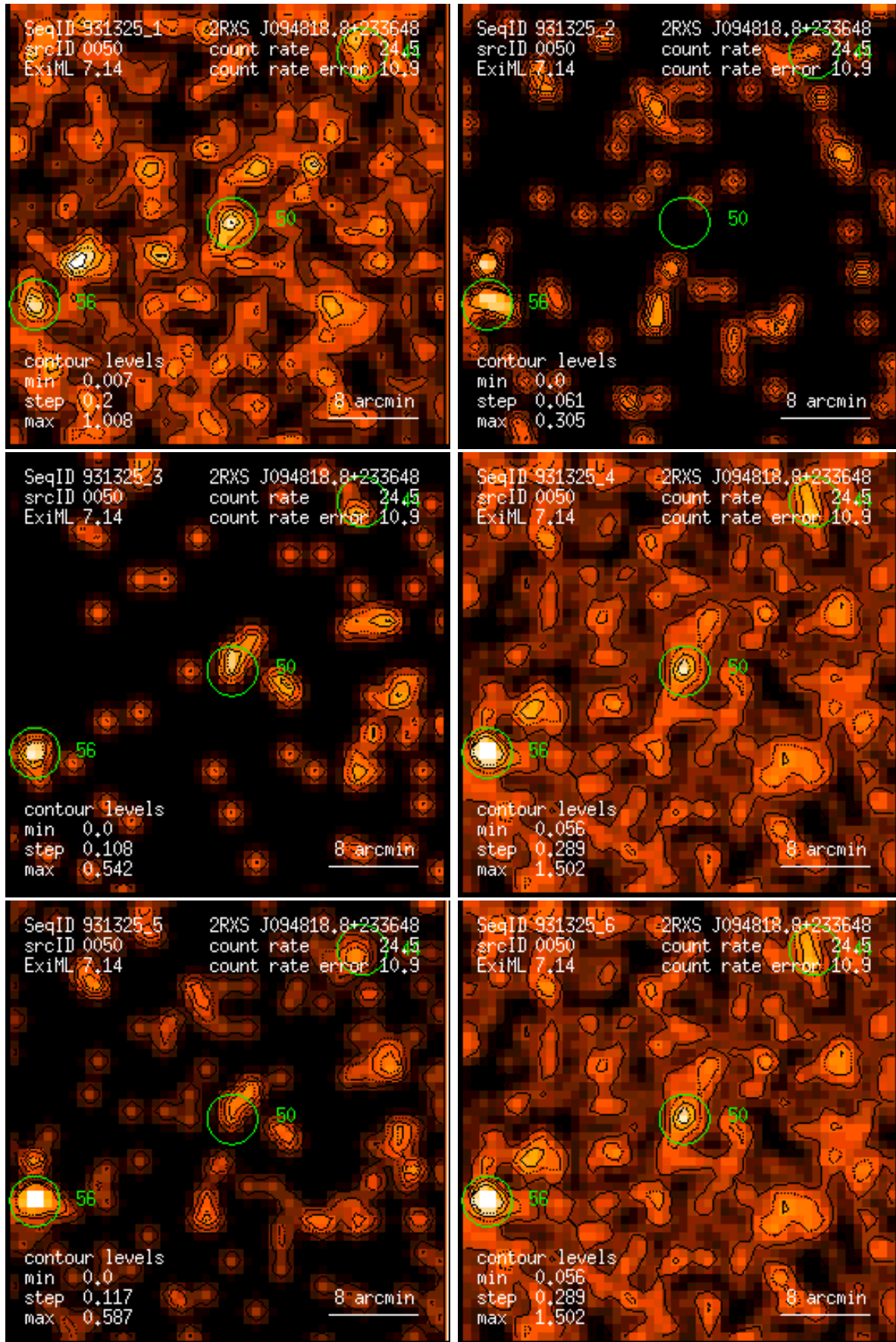
Figure 50: RASS 931325: detection 0050: band rate images, Gaussian filter: (1) PSPC channels 11 – 41, (2) 52 – 90, (3) 91 – 201, (4) 11 – 235, (5) 52 – 201, (6) 11 – 201. Broad band rates in counts/ks. Band rate contour levels in counts/ks/arcmin 2 .
