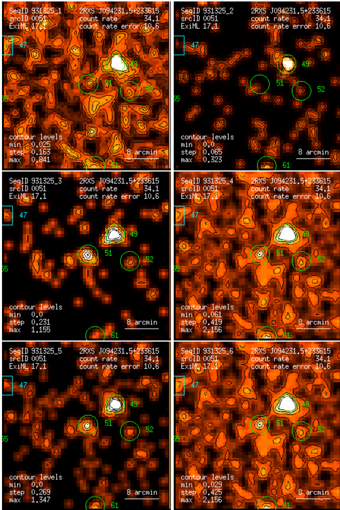
Figure 51: RASS 931325: detection 0051: band rate images, Gaussian filter: (1) PSPC channels 11 – 41, (2) 52 – 90, (3) 91 – 201, (4) 11 – 235, (5) 52 – 201, (6) 11 – 201. Broad band rates in counts/ks. Band rate contour levels in counts/ks/arcmin 2 .
