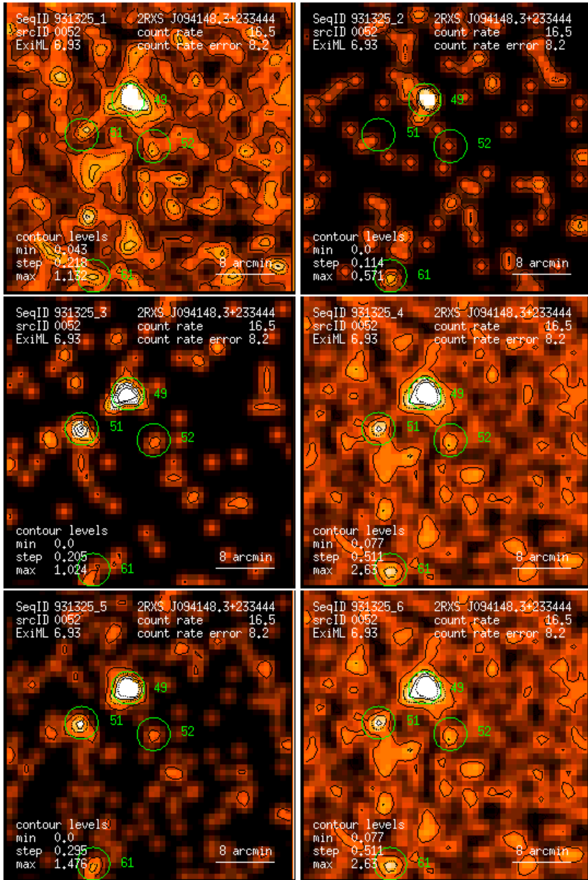
Figure 52: RASS 931325: detection 0052: band rate images, Gaussian filter: (1) PSPC channels 11 – 41, (2) 52 – 90, (3) 91 – 201, (4) 11 – 235, (5) 52 – 201, (6) 11 – 201. Broad band rates in counts/ks. Band rate contour levels in counts/ks/arcmin 2 .
