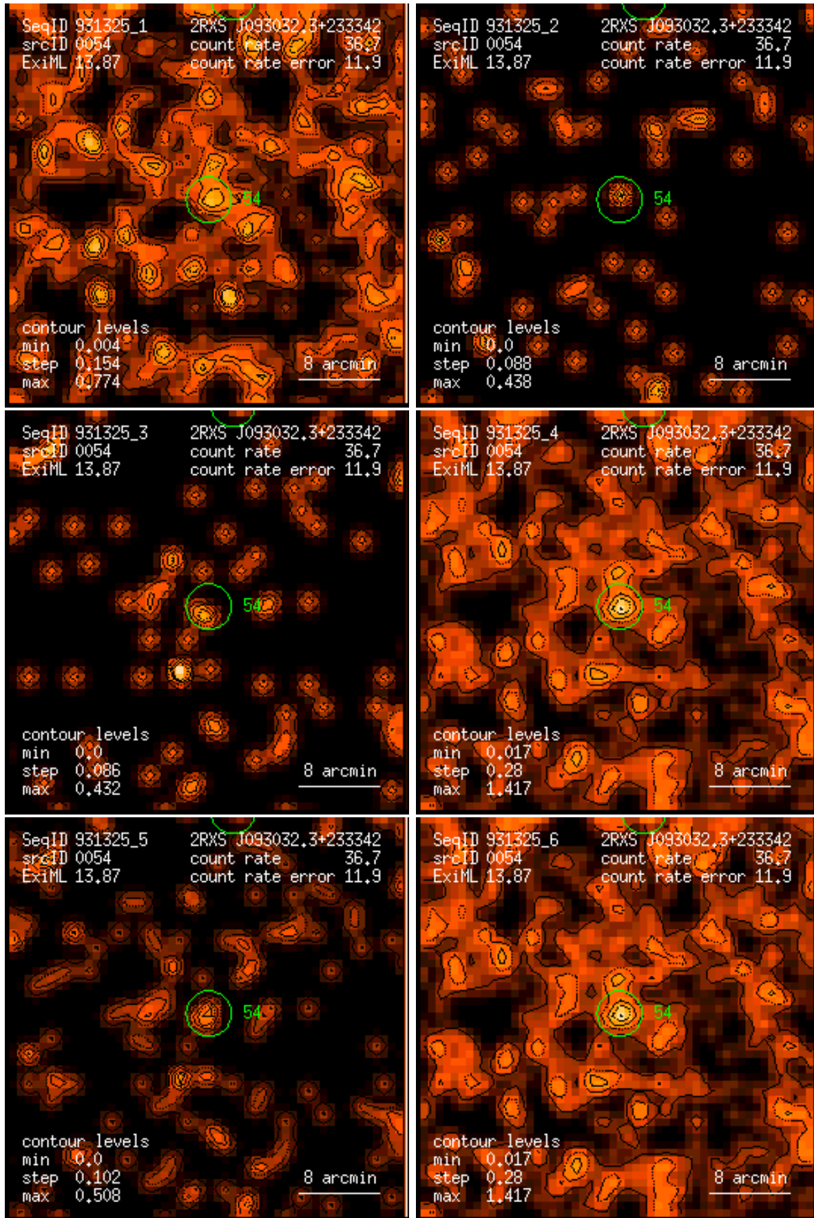
Figure 54: RASS 931325: detection 0054: band rate images, Gaussian filter: (1) PSPC channels 11 – 41, (2) 52 – 90, (3) 91 – 201, (4) 11 – 235, (5) 52 – 201, (6) 11 – 201. Broad band rates in counts/ks. Band rate contour levels in counts/ks/arcmin 2 .
