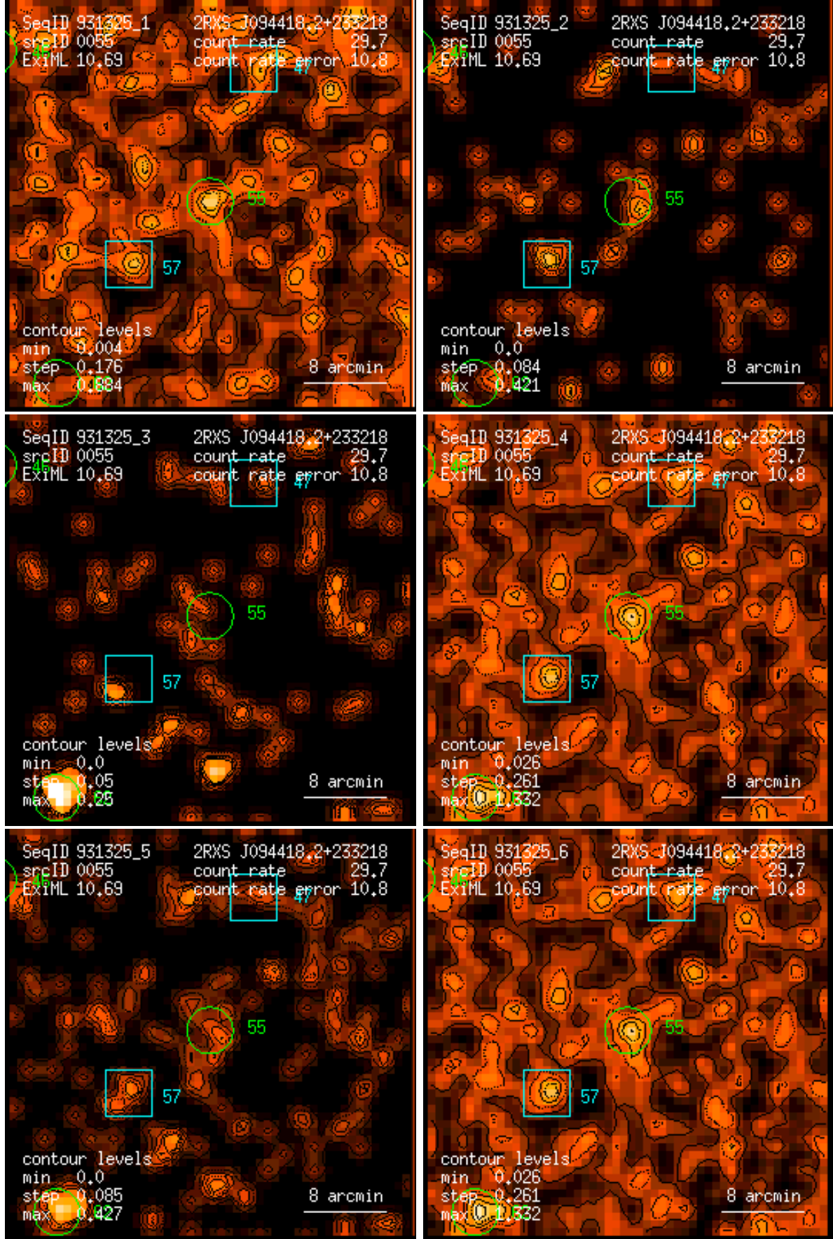
Figure 55: RASS 931325: detection 0055: band rate images, Gaussian filter: (1) PSPC channels 11 – 41, (2) 52 – 90, (3) 91 – 201, (4) 11 – 235, (5) 52 – 201, (6) 11 – 201. Broad band rates in counts/ks. Band rate contour levels in counts/ks/arcmin 2 .
