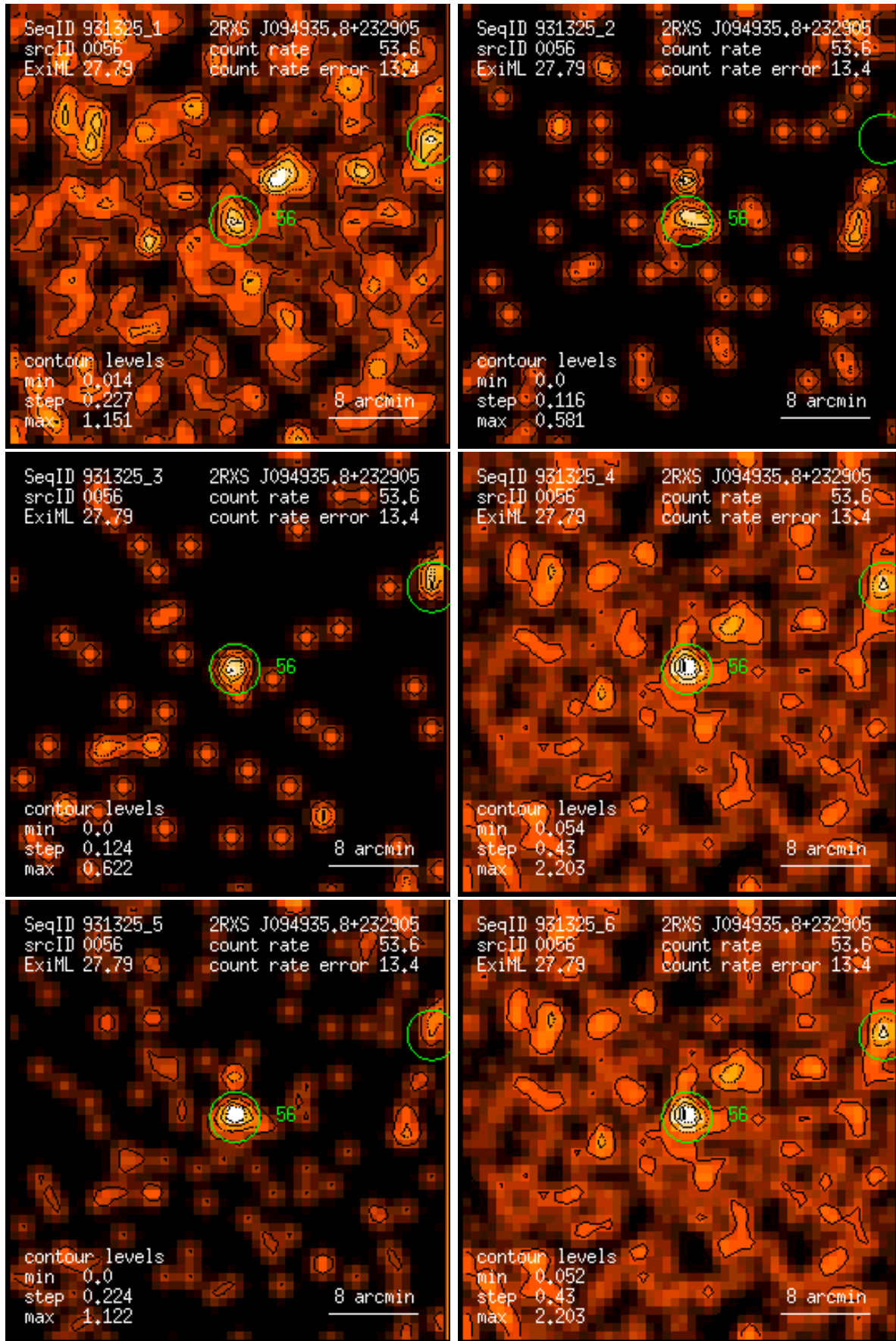
Figure 56: RASS 931325: detection 0056: band rate images, Gaussian filter: (1) PSPC channels 11 – 41, (2) 52 – 90, (3) 91 – 201, (4) 11 – 235, (5) 52 – 201, (6) 11 – 201. Broad band rates in counts/ks. Band rate contour levels in counts/ks/arcmin 2 .
