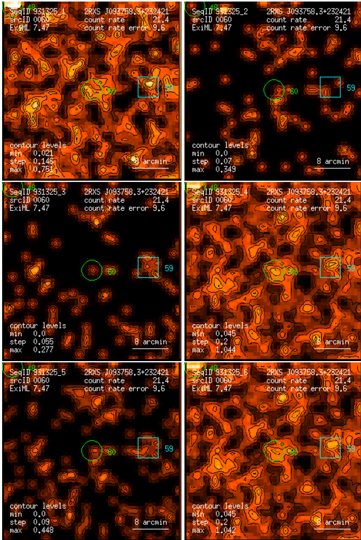
Figure 60: RASS 931325: detection 0060: band rate images, Gaussian filter: (1) PSPC channels 11 – 41, (2) 52 – 90, (3) 91 – 201, (4) 11 – 235, (5) 52 – 201, (6) 11 – 201. Broad band rates in counts/ks. Band rate contour levels in counts/ks/arcmin 2 .
