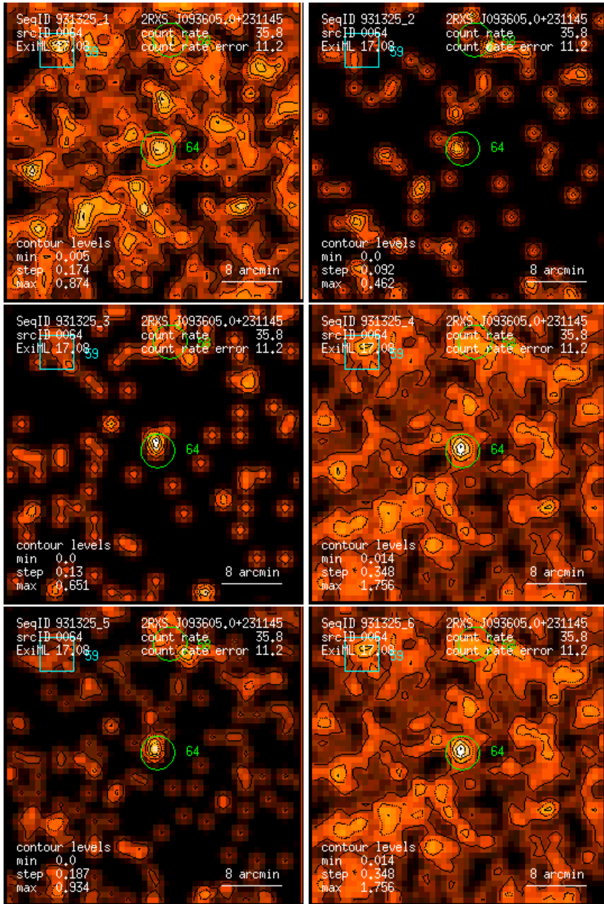
Figure 64: RASS 931325: detection 0064: band rate images, Gaussian filter: (1) PSPC channels 11 – 41, (2) 52 – 90, (3) 91 – 201, (4) 11 – 235, (5) 52 – 201, (6) 11 – 201. Broad band rates in counts/ks. Band rate contour levels in counts/ks/arcmin 2 .
