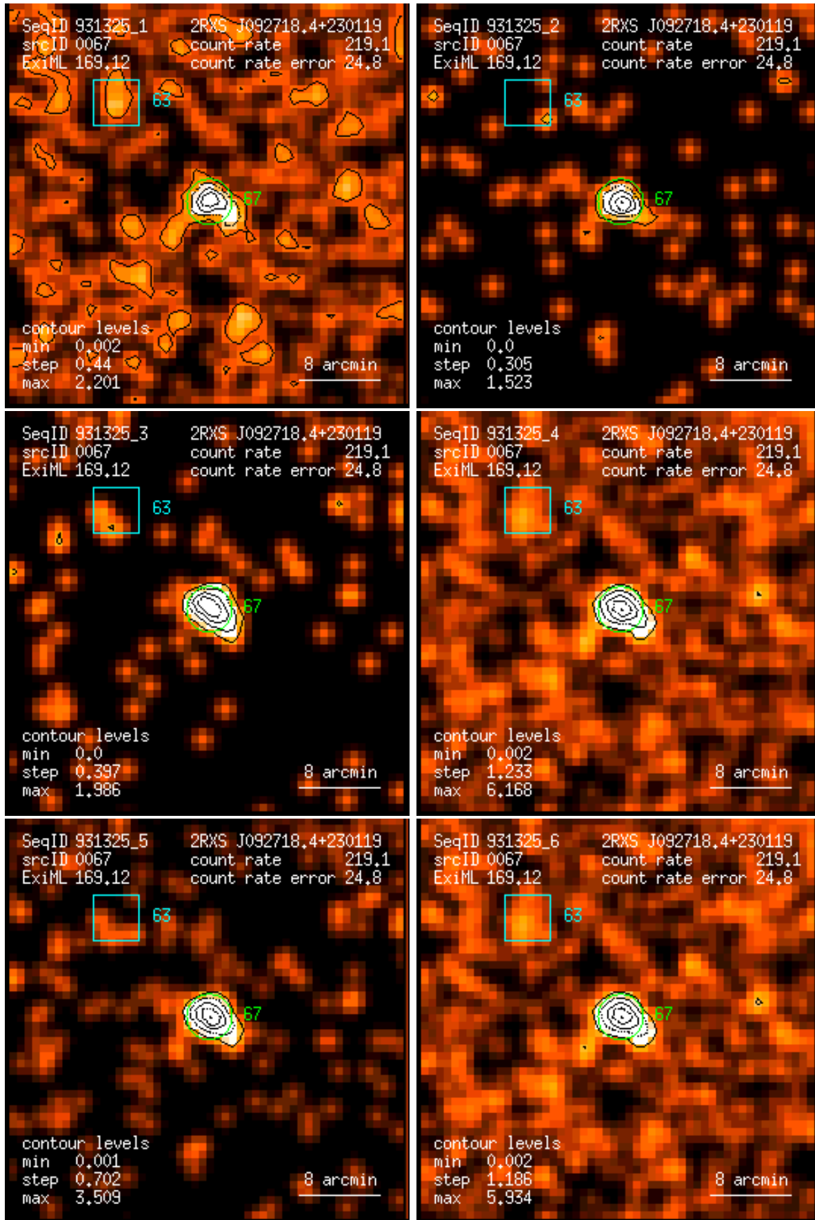
Figure 67: RASS 931325: detection 0067: band rate images, Gaussian filter: (1) PSPC channels 11 – 41, (2) 52 – 90, (3) 91 – 201, (4) 11 – 235, (5) 52 – 201, (6) 11 – 201. Broad band rates in counts/ks. Band rate contour levels in counts/ks/arcmin 2 .
