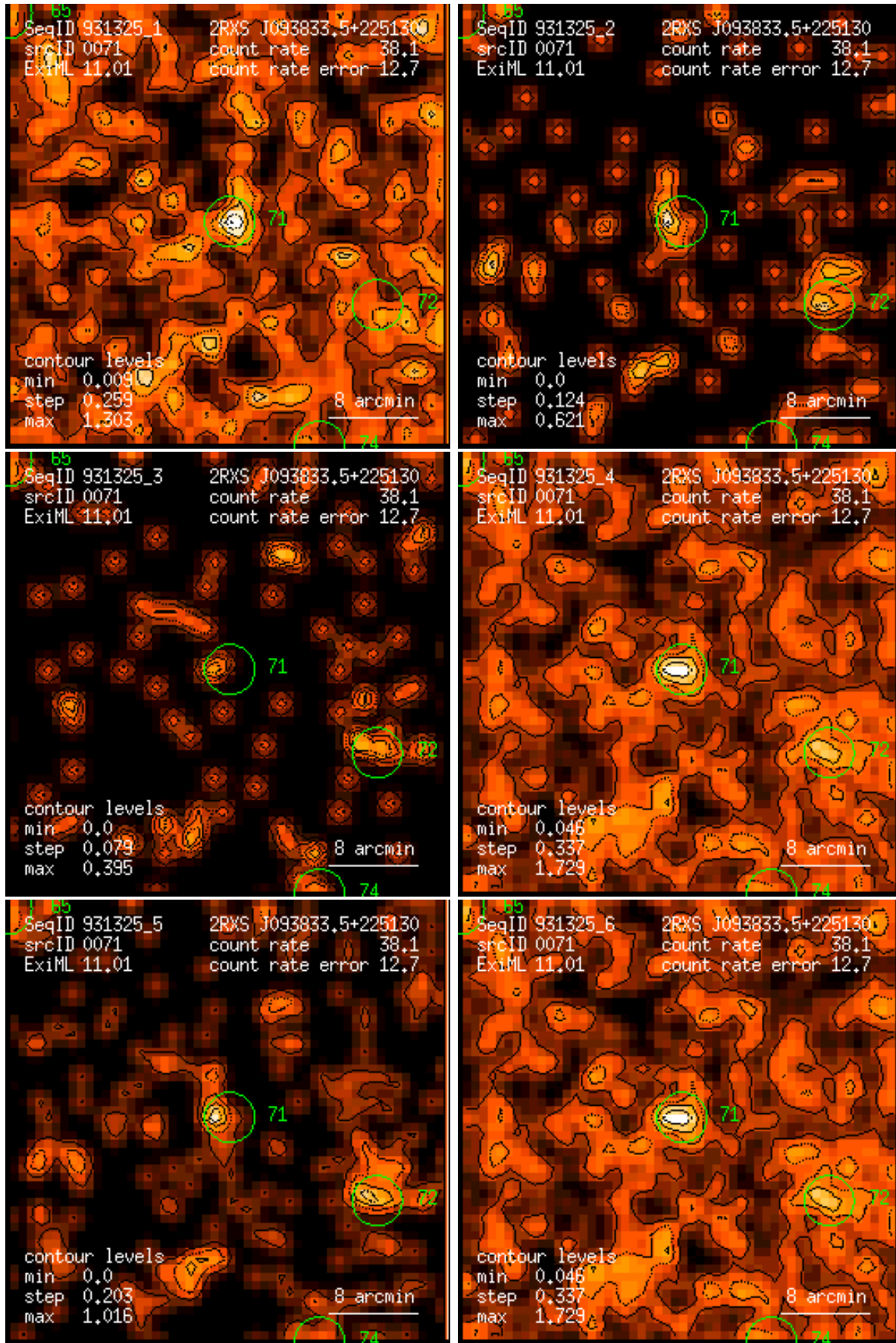
Figure 71: RASS 931325: detection 0071: band rate images, Gaussian filter: (1) PSPC channels 11 – 41, (2) 52 – 90, (3) 91 – 201, (4) 11 – 235, (5) 52 – 201, (6) 11 – 201. Broad band rates in counts/ks. Band rate contour levels in counts/ks/arcmin 2 .
