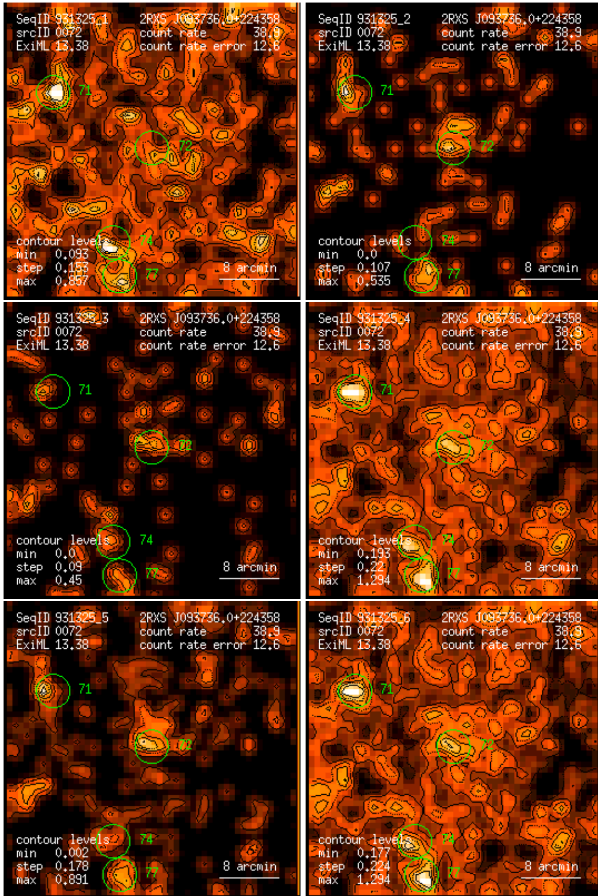
Figure 72: RASS 931325: detection 0072: band rate images, Gaussian filter: (1) PSPC channels 11 – 41, (2) 52 – 90, (3) 91 – 201, (4) 11 – 235, (5) 52 – 201, (6) 11 – 201. Broad band rates in counts/ks. Band rate contour levels in counts/ks/arcmin 2 .
