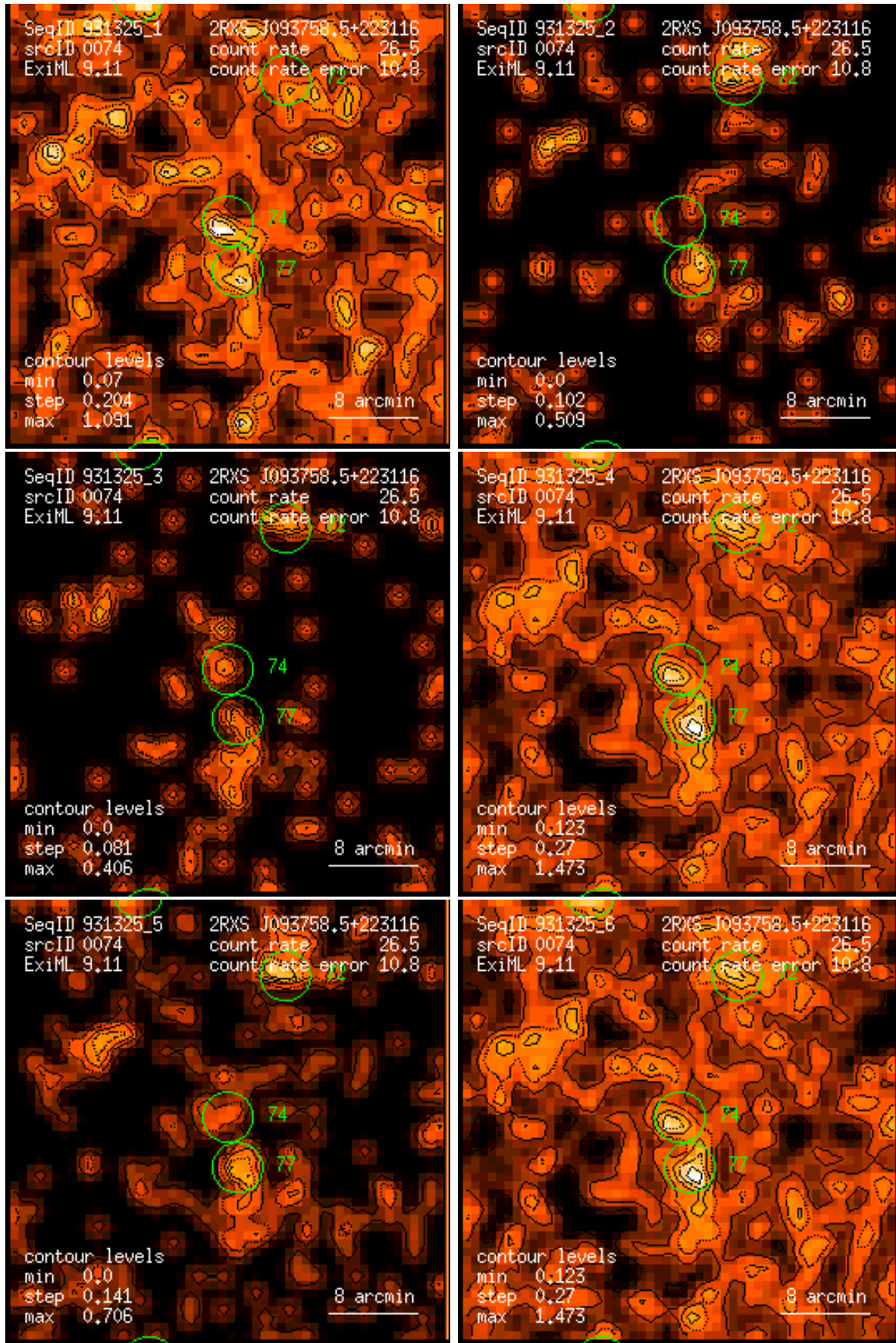
Figure 74: RASS 931325: detection 0074: band rate images, Gaussian filter: (1) PSPC channels 11 – 41, (2) 52 – 90, (3) 91 – 201, (4) 11 – 235, (5) 52 – 201, (6) 11 – 201. Broad band rates in counts/ks. Band rate contour levels in counts/ks/arcmin 2 .
