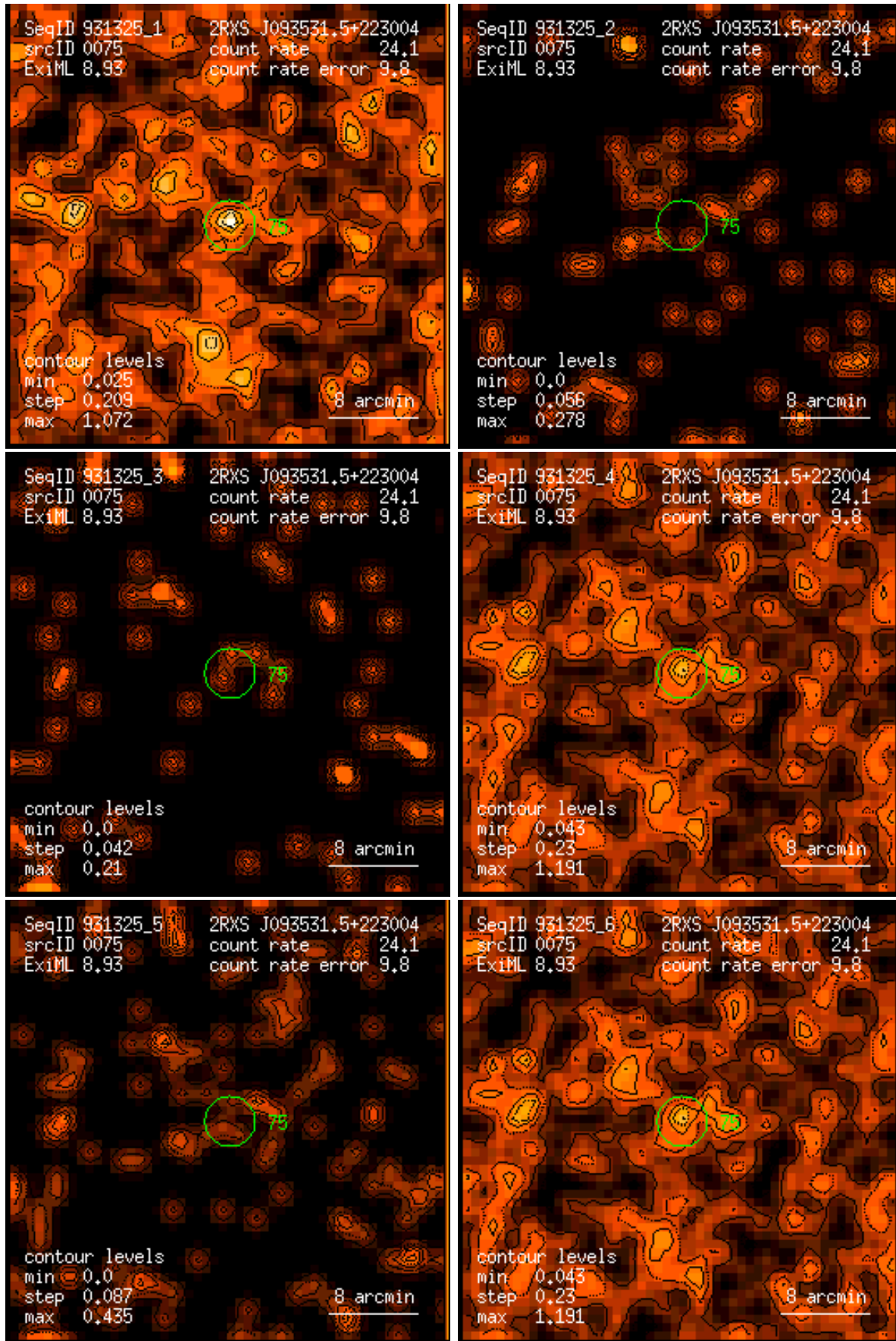
Figure 75: RASS 931325: detection 0075: band rate images, Gaussian filter: (1) PSPC channels 11 – 41, (2) 52 – 90, (3) 91 – 201, (4) 11 – 235, (5) 52 – 201, (6) 11 – 201. Broad band rates in counts/ks. Band rate contour levels in counts/ks/arcmin 2 .
