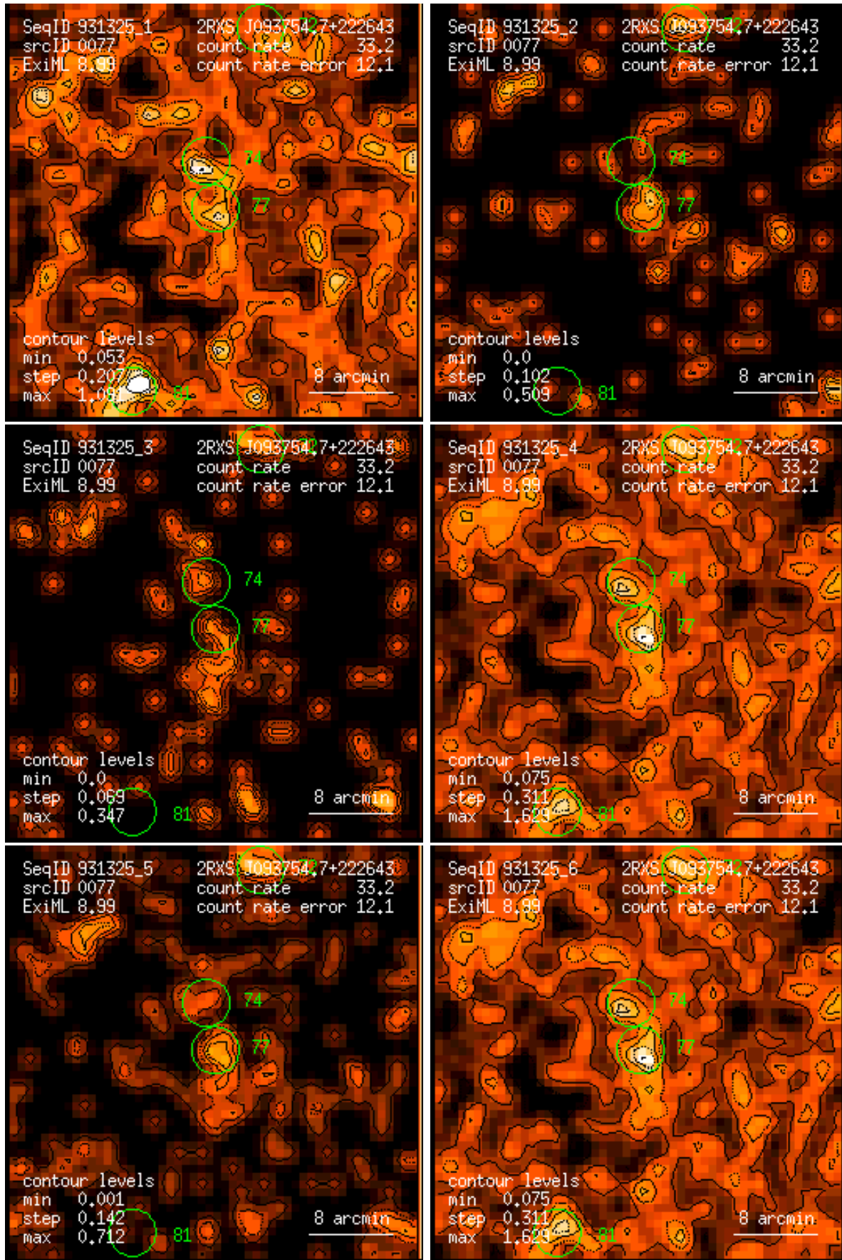
Figure 77: RASS 931325: detection 0077: band rate images, Gaussian filter: (1) PSPC channels 11 – 41, (2) 52 – 90, (3) 91 – 201, (4) 11 – 235, (5) 52 – 201, (6) 11 – 201. Broad band rates in counts/ks. Band rate contour levels in counts/ks/arcmin 2 .
