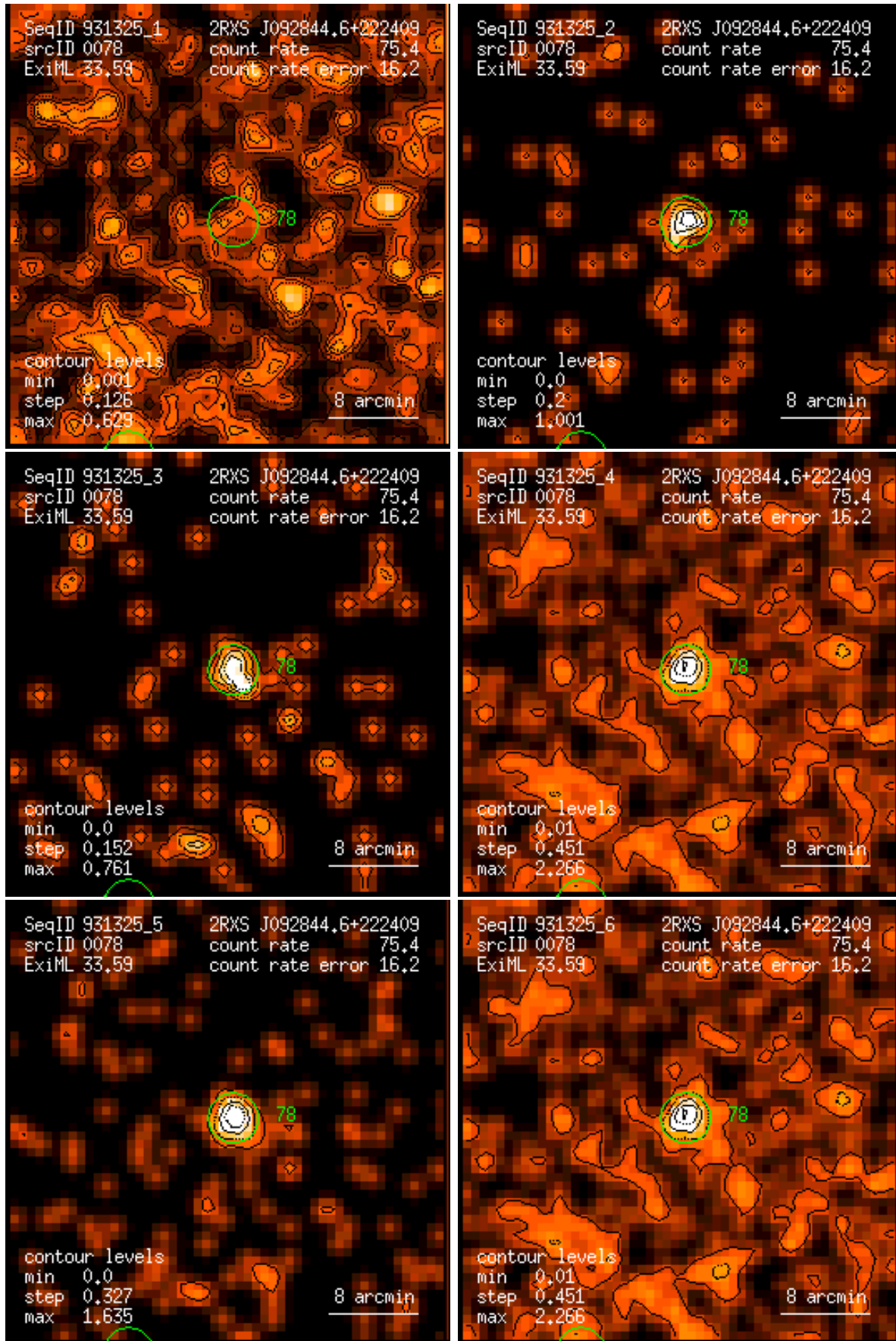
Figure 78: RASS 931325: detection 0078: band rate images, Gaussian filter: (1) PSPC channels 11 – 41, (2) 52 – 90, (3) 91 – 201, (4) 11 – 235, (5) 52 – 201, (6) 11 – 201. Broad band rates in counts/ks. Band rate contour levels in counts/ks/arcmin 2 .
