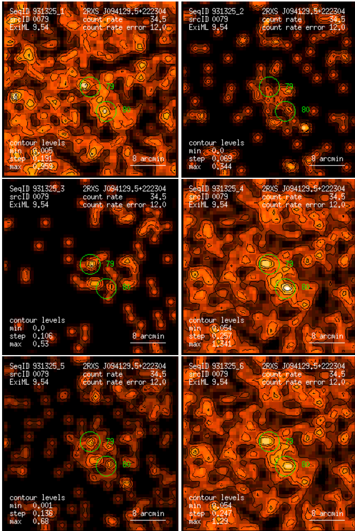
Figure 79: RASS 931325: detection 0079: band rate images, Gaussian filter: (1) PSPC channels 11 – 41, (2) 52 – 90, (3) 91 – 201, (4) 11 – 235, (5) 52 – 201, (6) 11 – 201. Broad band rates in counts/ks. Band rate contour levels in counts/ks/arcmin 2 .
