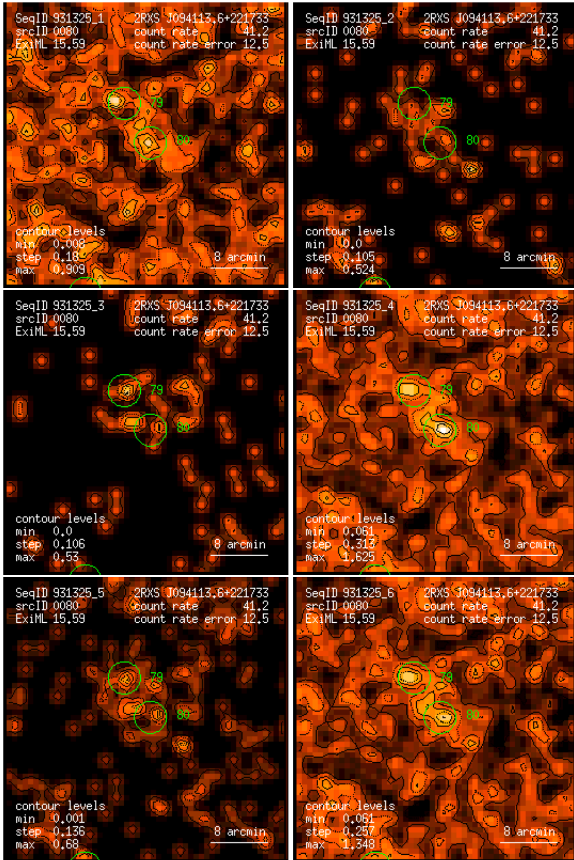
Figure 80: RASS 931325: detection 0080: band rate images, Gaussian filter: (1) PSPC channels 11 – 41, (2) 52 – 90, (3) 91 – 201, (4) 11 – 235, (5) 52 – 201, (6) 11 – 201. Broad band rates in counts/ks. Band rate contour levels in counts/ks/arcmin 2 .
