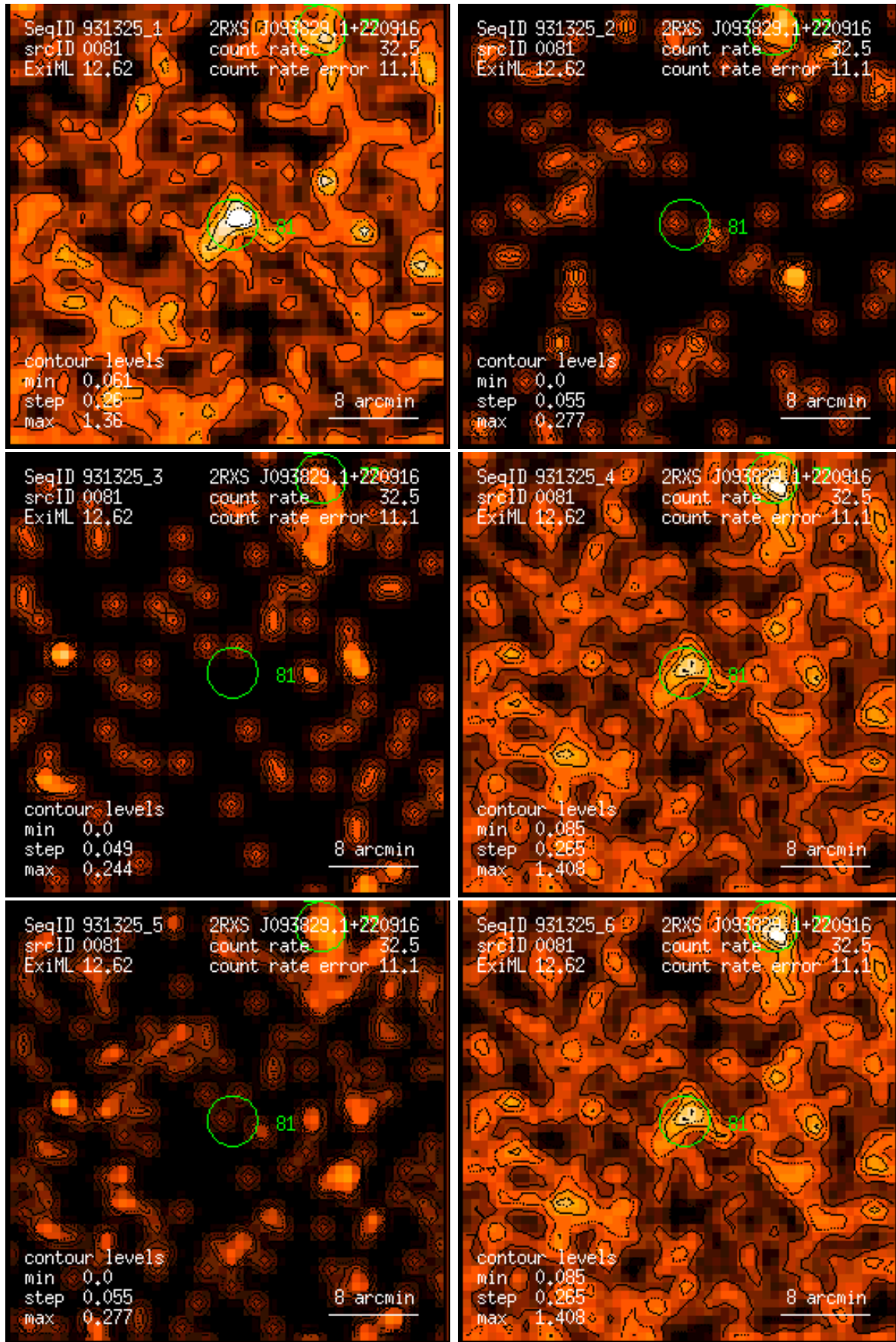
Figure 81: RASS 931325: detection 0081: band rate images, Gaussian filter: (1) PSPC channels 11 – 41, (2) 52 – 90, (3) 91 – 201, (4) 11 – 235, (5) 52 – 201, (6) 11 – 201. Broad band rates in counts/ks. Band rate contour levels in counts/ks/arcmin 2 .
