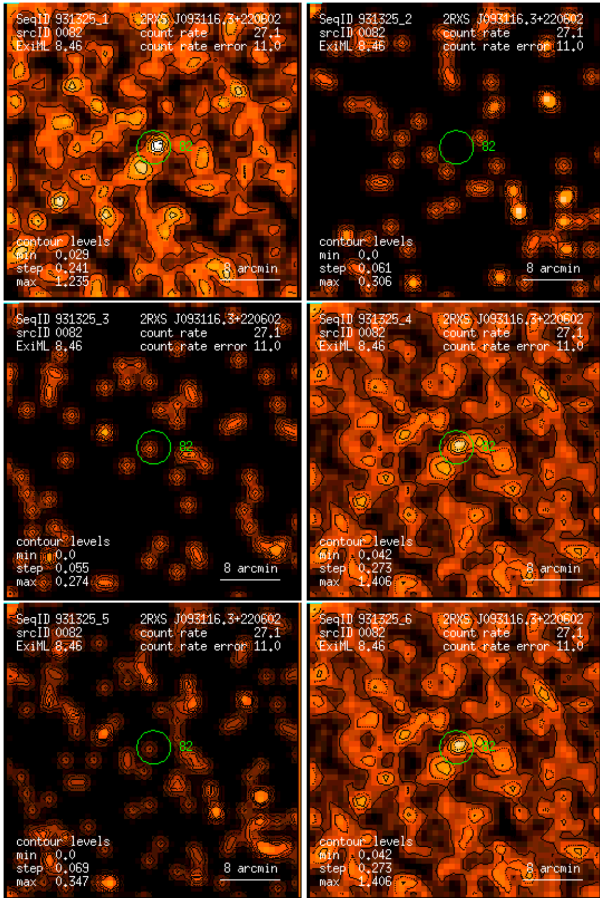
Figure 82: RASS 931325: detection 0082: band rate images, Gaussian filter: (1) PSPC channels 11 – 41, (2) 52 – 90, (3) 91 – 201, (4) 11 – 235, (5) 52 – 201, (6) 11 – 201. Broad band rates in counts/ks. Band rate contour levels in counts/ks/arcmin 2 .
