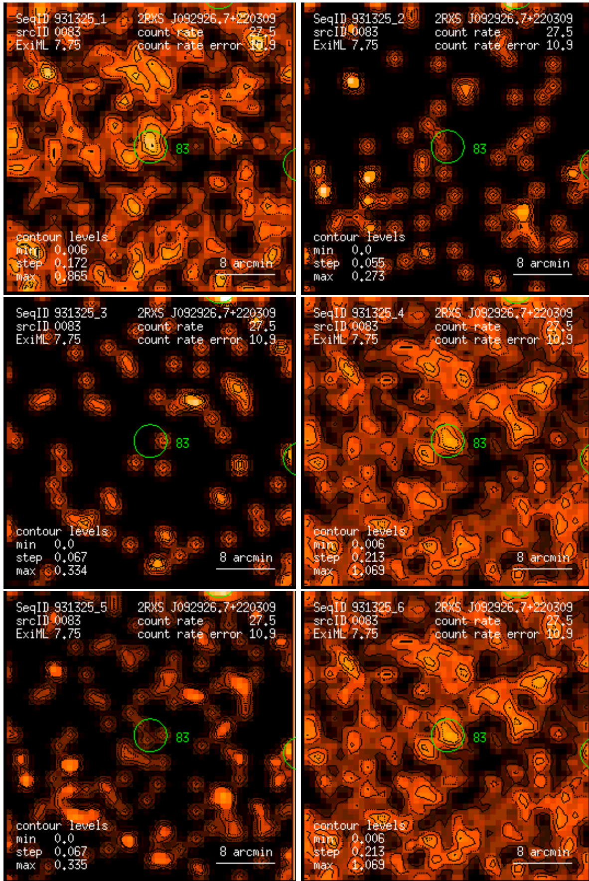
Figure 83: RASS 931325: detection 0083: band rate images, Gaussian filter: (1) PSPC channels 11 – 41, (2) 52 – 90, (3) 91 – 201, (4) 11 – 235, (5) 52 – 201, (6) 11 – 201. Broad band rates in counts/ks. Band rate contour levels in counts/ks/arcmin 2 .
