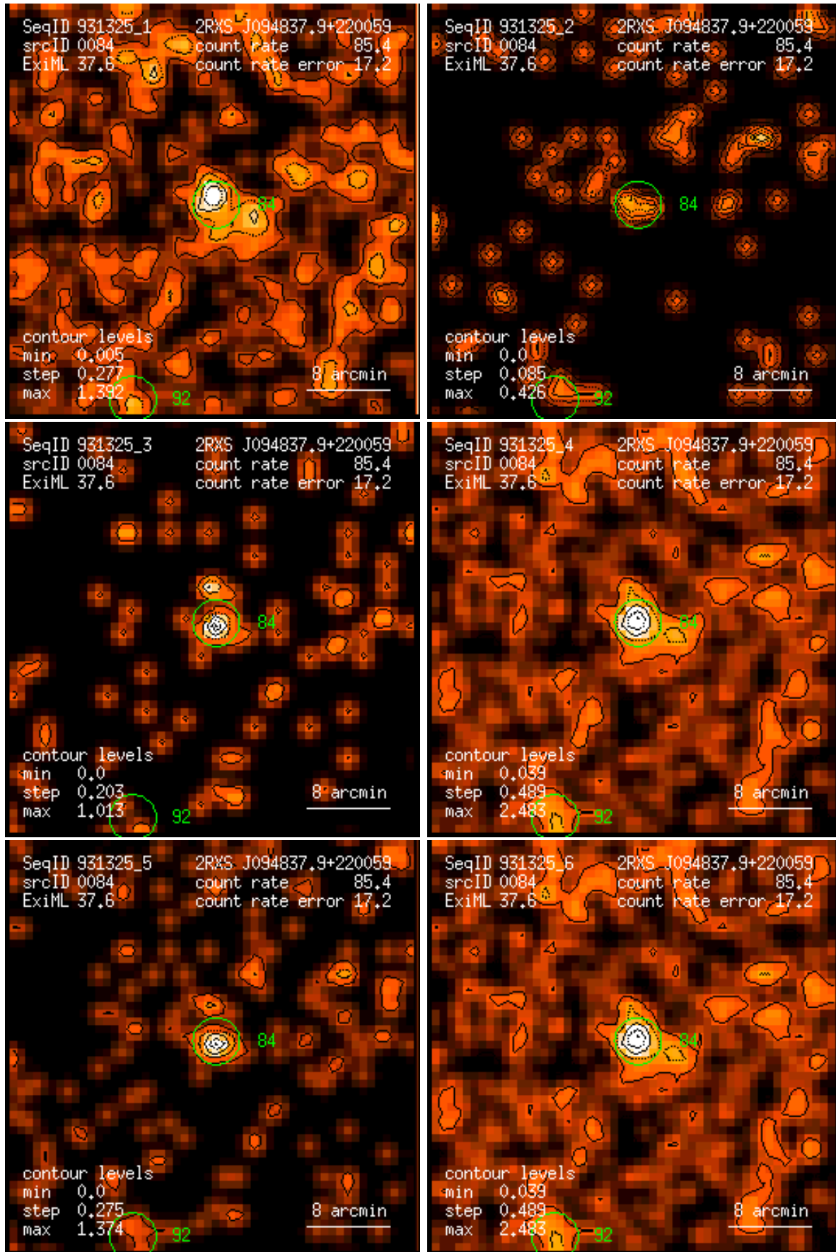
Figure 84: RASS 931325: detection 0084: band rate images, Gaussian filter: (1) PSPC channels 11 – 41, (2) 52 – 90, (3) 91 – 201, (4) 11 – 235, (5) 52 – 201, (6) 11 – 201. Broad band rates in counts/ks. Band rate contour levels in counts/ks/arcmin 2 .
