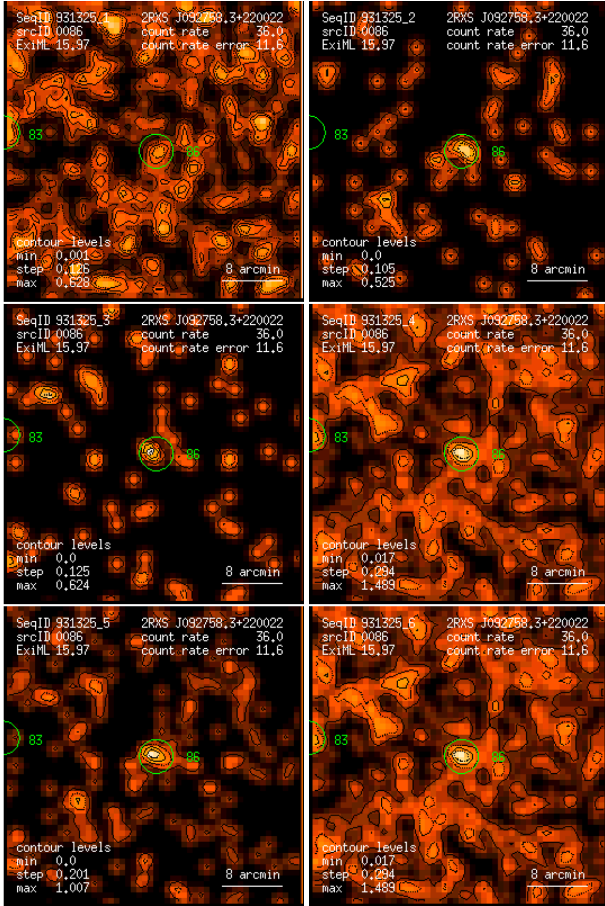
Figure 86: RASS 931325: detection 0086: band rate images, Gaussian filter: (1) PSPC channels 11 – 41, (2) 52 – 90, (3) 91 – 201, (4) 11 – 235, (5) 52 – 201, (6) 11 – 201. Broad band rates in counts/ks. Band rate contour levels in counts/ks/arcmin 2 .
