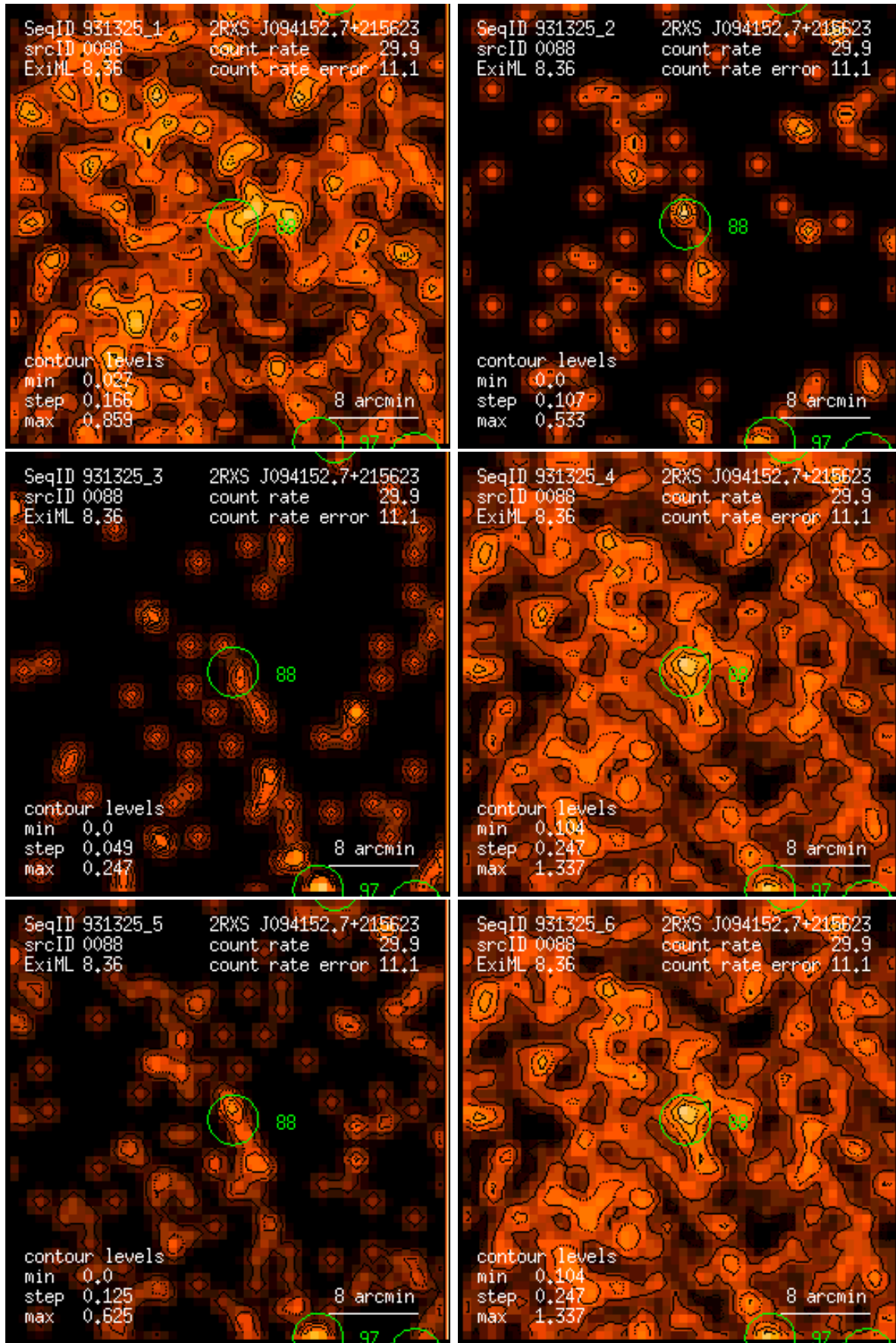
Figure 88: RASS 931325: detection 0088: band rate images, Gaussian filter: (1) PSPC channels 11 – 41, (2) 52 – 90, (3) 91 – 201, (4) 11 – 235, (5) 52 – 201, (6) 11 – 201. Broad band rates in counts/ks. Band rate contour levels in counts/ks/arcmin 2 .
