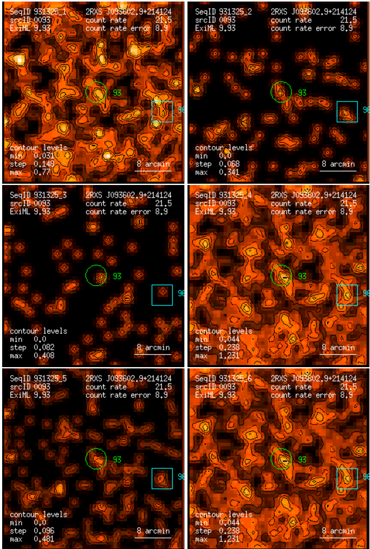
Figure 93: RASS 931325: detection 0093: band rate images, Gaussian filter: (1) PSPC channels 11 – 41, (2) 52 – 90, (3) 91 – 201, (4) 11 – 235, (5) 52 – 201, (6) 11 – 201. Broad band rates in counts/ks. Band rate contour levels in counts/ks/arcmin 2 .
