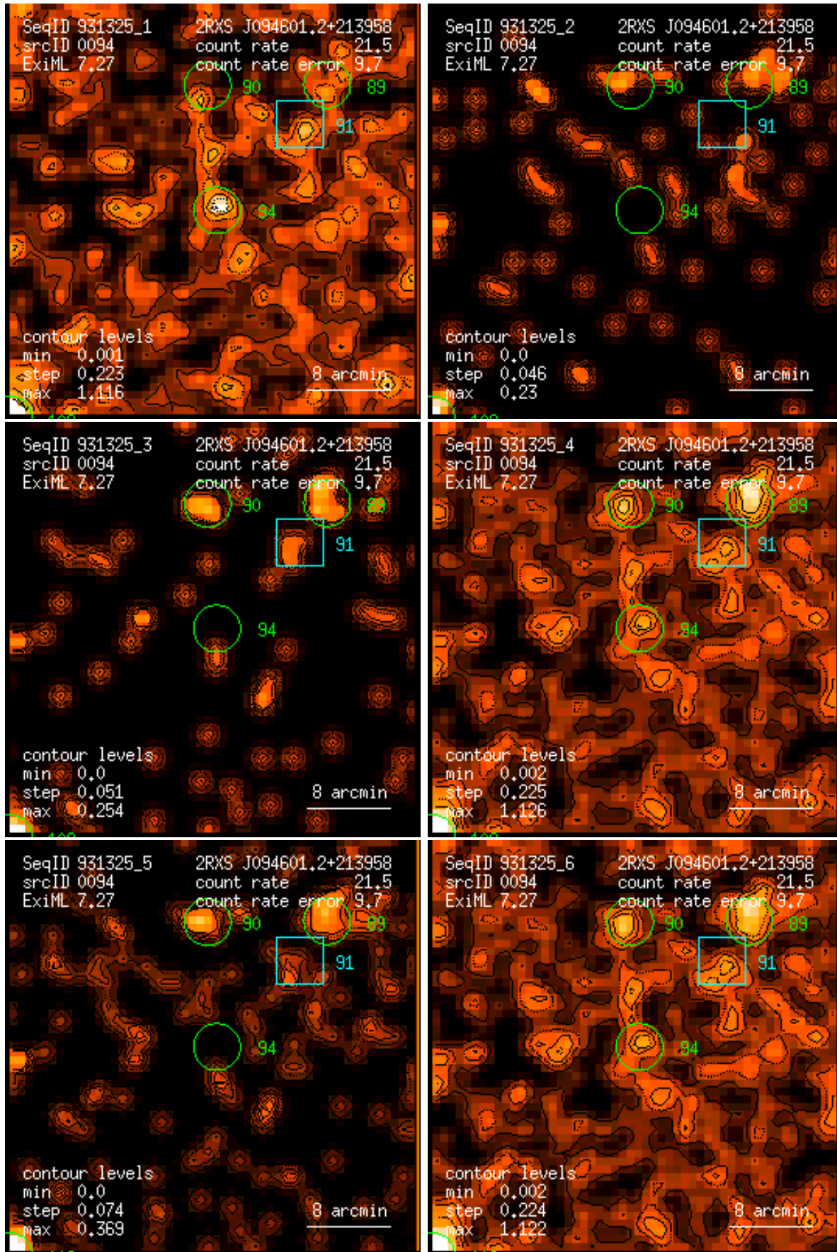
Figure 94: RASS 931325: detection 0094: band rate images, Gaussian filter: (1) PSPC channels 11 – 41, (2) 52 – 90, (3) 91 – 201, (4) 11 – 235, (5) 52 – 201, (6) 11 – 201. Broad band rates in counts/ks. Band rate contour levels in counts/ks/arcmin 2 .
