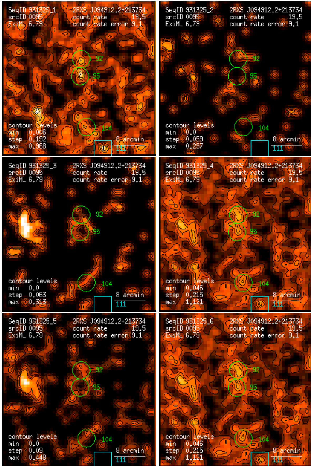
Figure 95: RASS 931325: detection 0095: band rate images, Gaussian filter: (1) PSPC channels 11 – 41, (2) 52 – 90, (3) 91 – 201, (4) 11 – 235, (5) 52 – 201, (6) 11 – 201. Broad band rates in counts/ks. Band rate contour levels in counts/ks/arcmin 2 .
