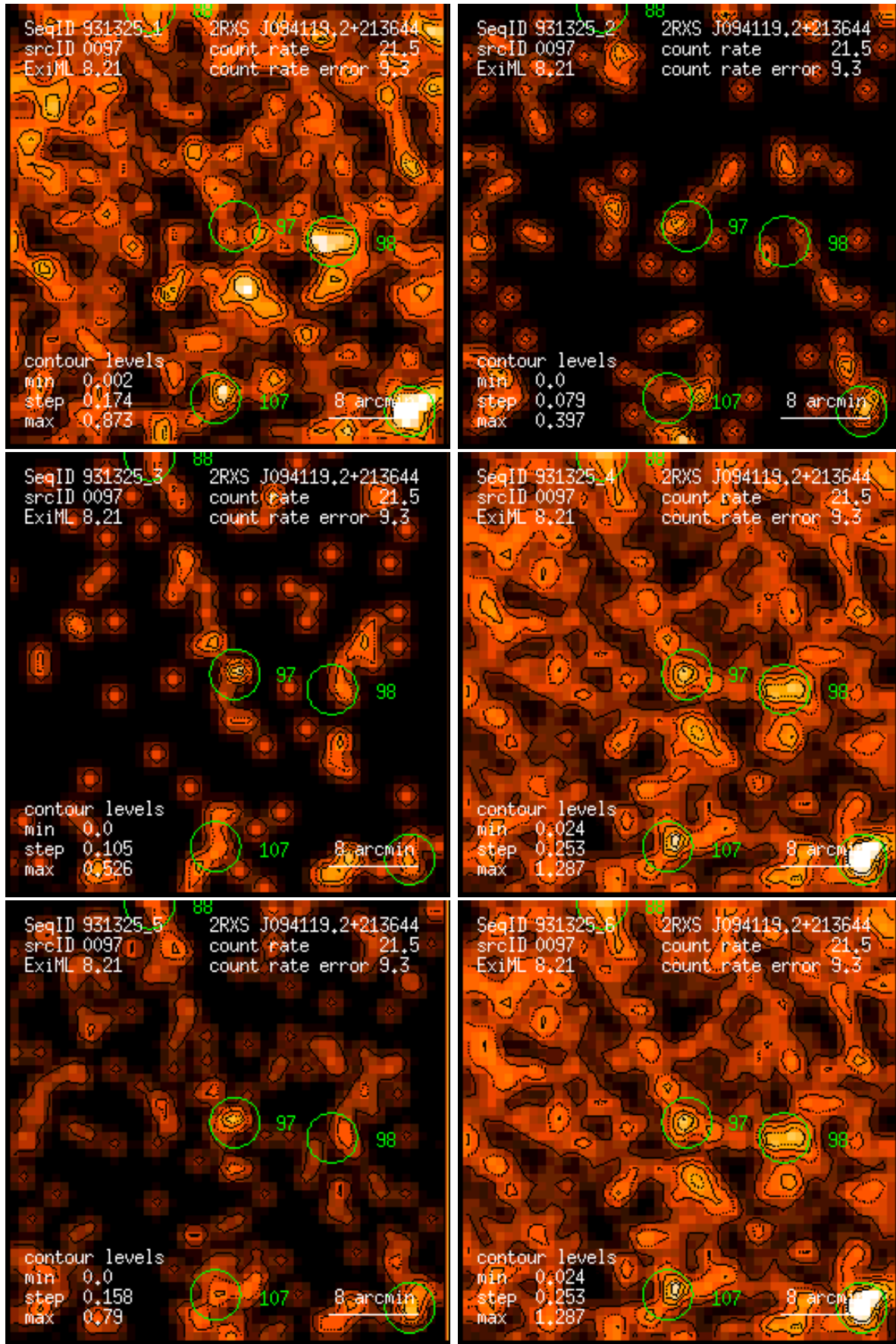
Figure 97: RASS 931325: detection 0097: band rate images, Gaussian filter: (1) PSPC channels 11 – 41, (2) 52 – 90, (3) 91 – 201, (4) 11 – 235, (5) 52 – 201, (6) 11 – 201. Broad band rates in counts/ks. Band rate contour levels in counts/ks/arcmin 2 .
