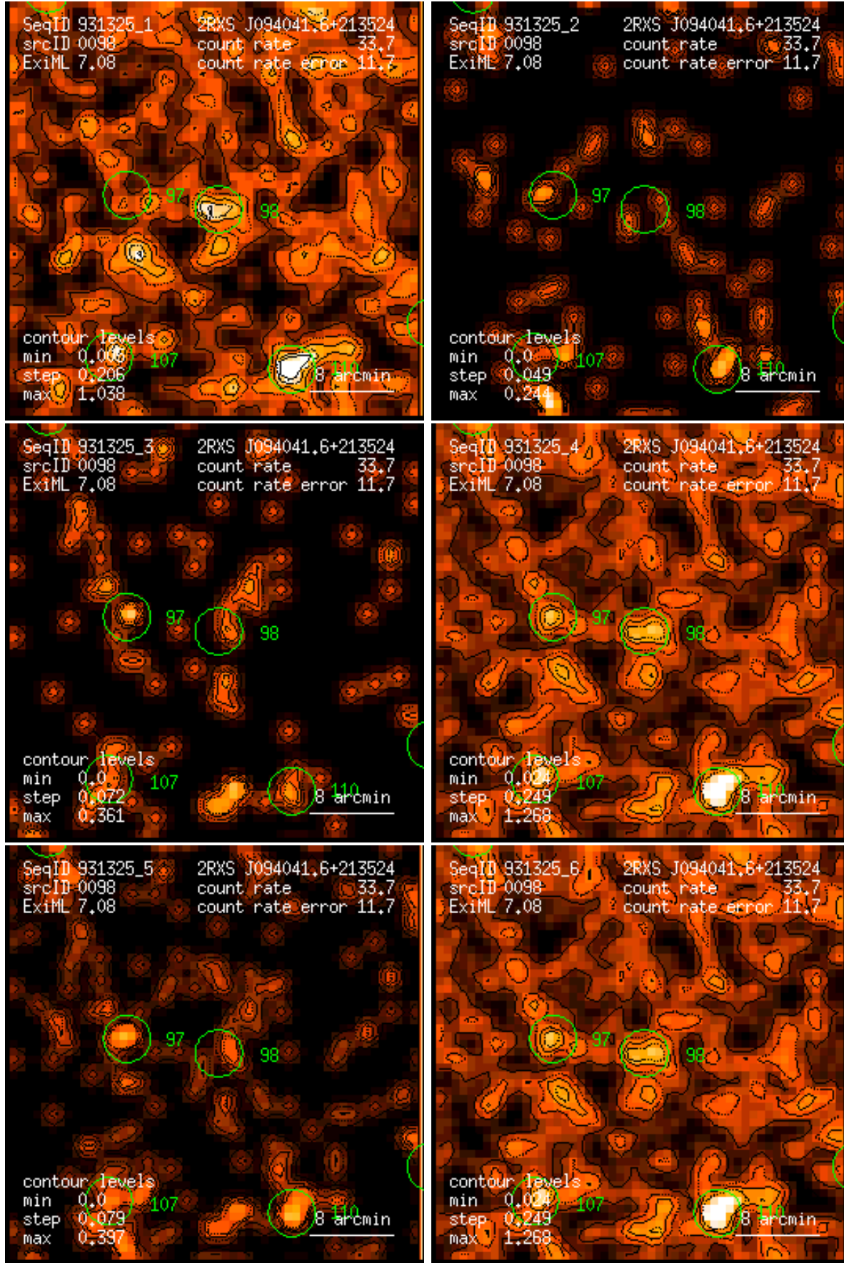
Figure 98: RASS 931325: detection 0098: band rate images, Gaussian filter: (1) PSPC channels 11 – 41, (2) 52 – 90, (3) 91 – 201, (4) 11 – 235, (5) 52 – 201, (6) 11 – 201. Broad band rates in counts/ks. Band rate contour levels in counts/ks/arcmin 2 .
