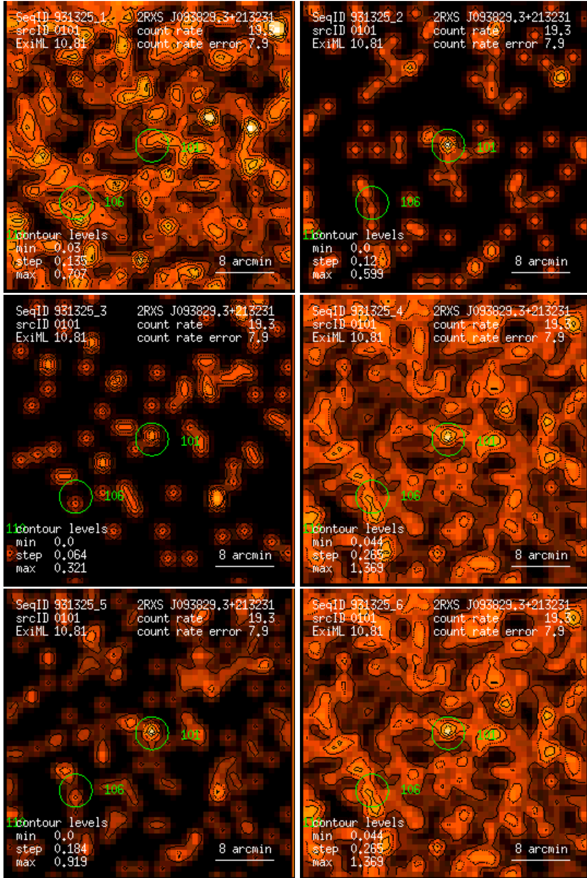
Figure 101: RASS 931325: detection 0101: band rate images, Gaussian filter: (1) PSPC channels 11 – 41, (2) 52 – 90, (3) 91 – 201, (4) 11 – 235, (5) 52 – 201, (6) 11 – 201. Broad band rates in counts/ks. Band rate contour levels in counts/ks/arcmin 2 .
