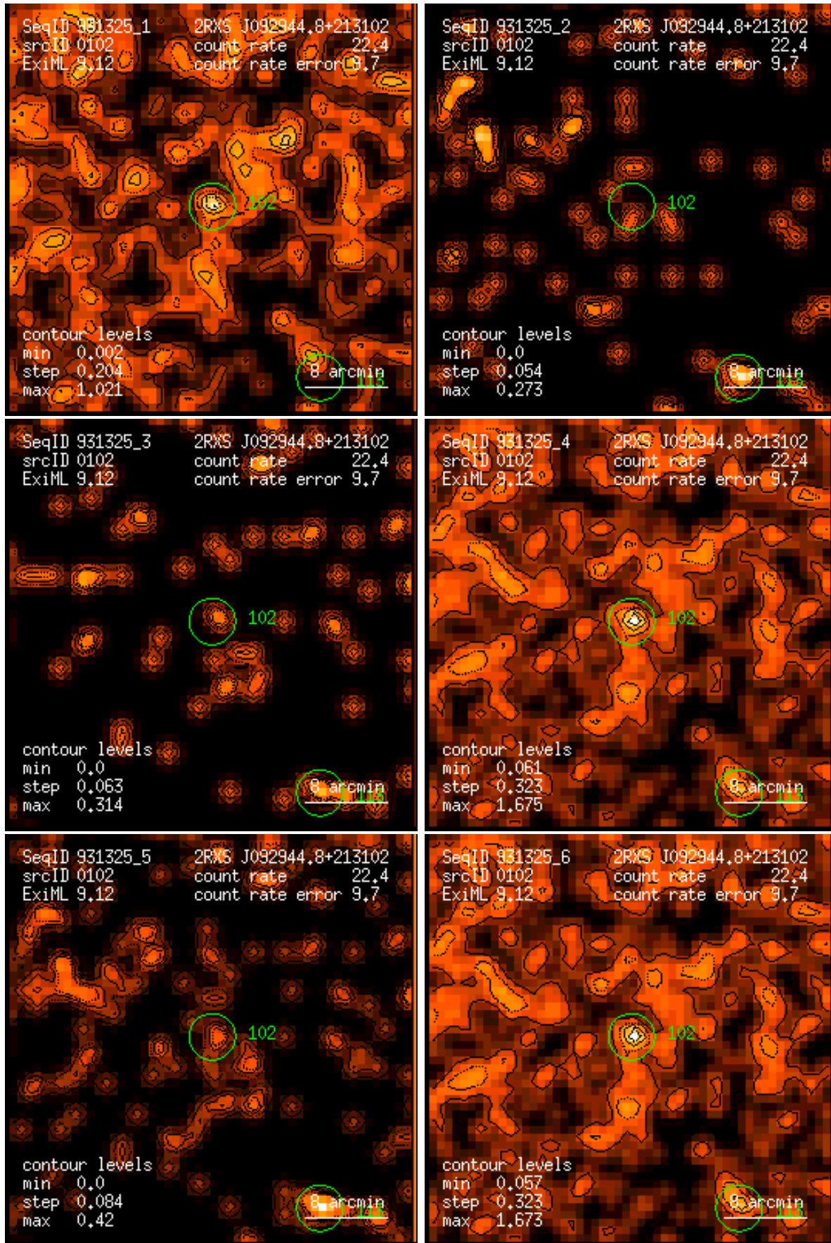
Figure 102: RASS 931325: detection 0102: band rate images, Gaussian filter: (1) PSPC channels 11 – 41, (2) 52 – 90, (3) 91 – 201, (4) 11 – 235, (5) 52 – 201, (6) 11 – 201. Broad band rates in counts/ks. Band rate contour levels in counts/ks/arcmin 2 .
