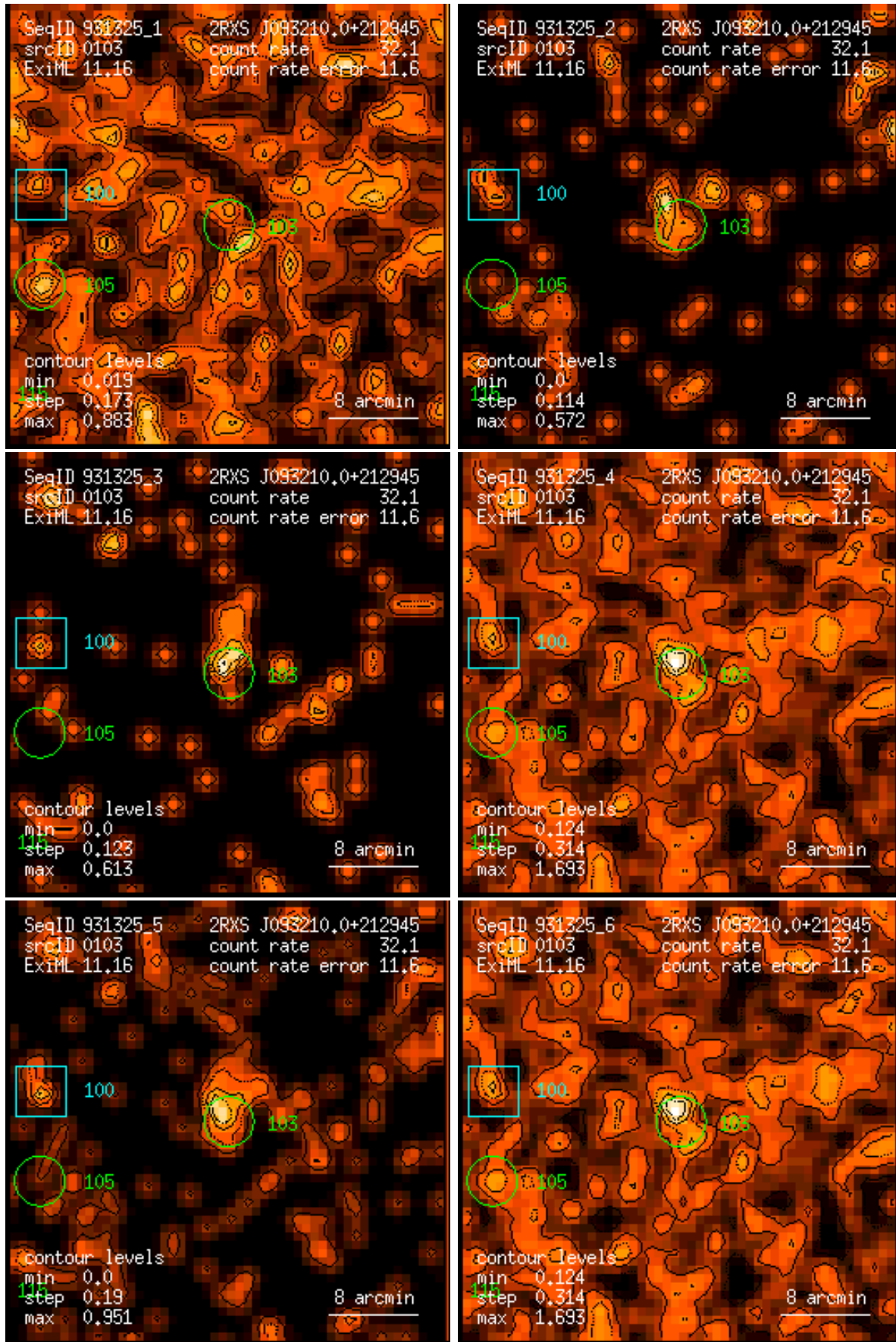
Figure 103: RASS 931325: detection 0103: band rate images, Gaussian filter: (1) PSPC channels 11 – 41, (2) 52 – 90, (3) 91 – 201, (4) 11 – 235, (5) 52 – 201, (6) 11 – 201. Broad band rates in counts/ks. Band rate contour levels in counts/ks/arcmin 2 .
