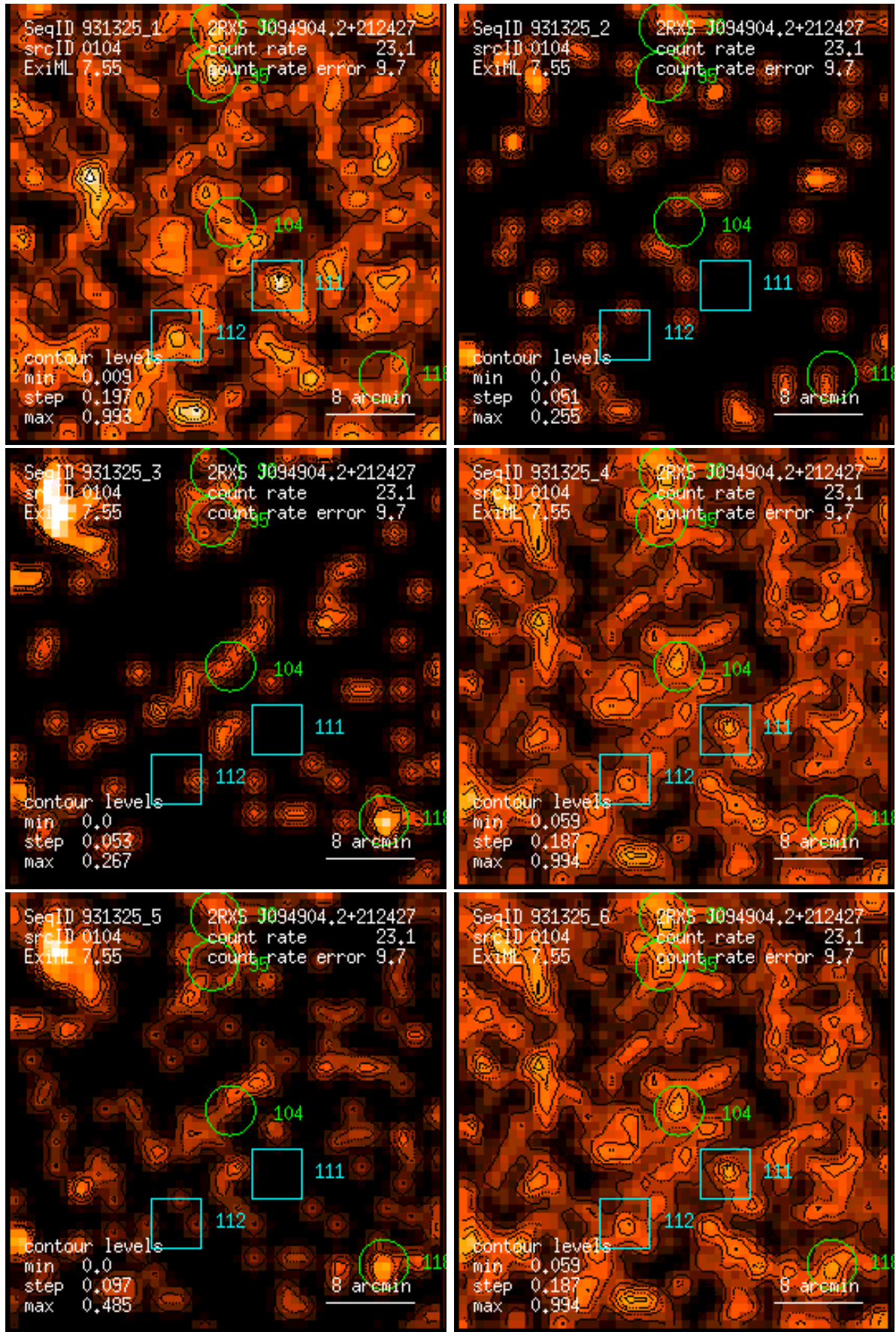
Figure 104: RASS 931325: detection 0104: band rate images, Gaussian filter: (1) PSPC channels 11 – 41, (2) 52 – 90, (3) 91 – 201, (4) 11 – 235, (5) 52 – 201, (6) 11 – 201. Broad band rates in counts/ks. Band rate contour levels in counts/ks/arcmin 2 .
