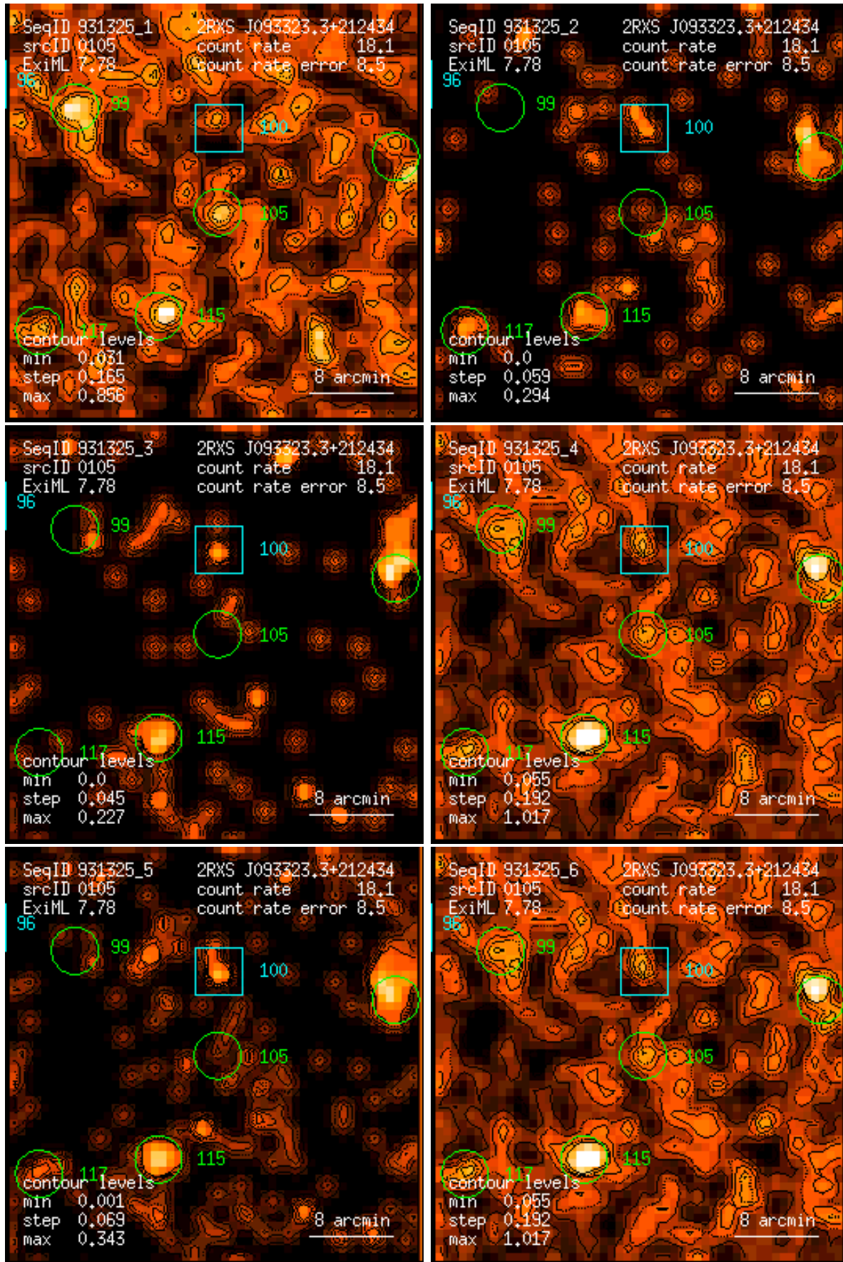
Figure 105: RASS 931325: detection 0105: band rate images, Gaussian filter: (1) PSPC channels 11 – 41, (2) 52 – 90, (3) 91 – 201, (4) 11 – 235, (5) 52 – 201, (6) 11 – 201. Broad band rates in counts/ks. Band rate contour levels in counts/ks/arcmin 2 .
