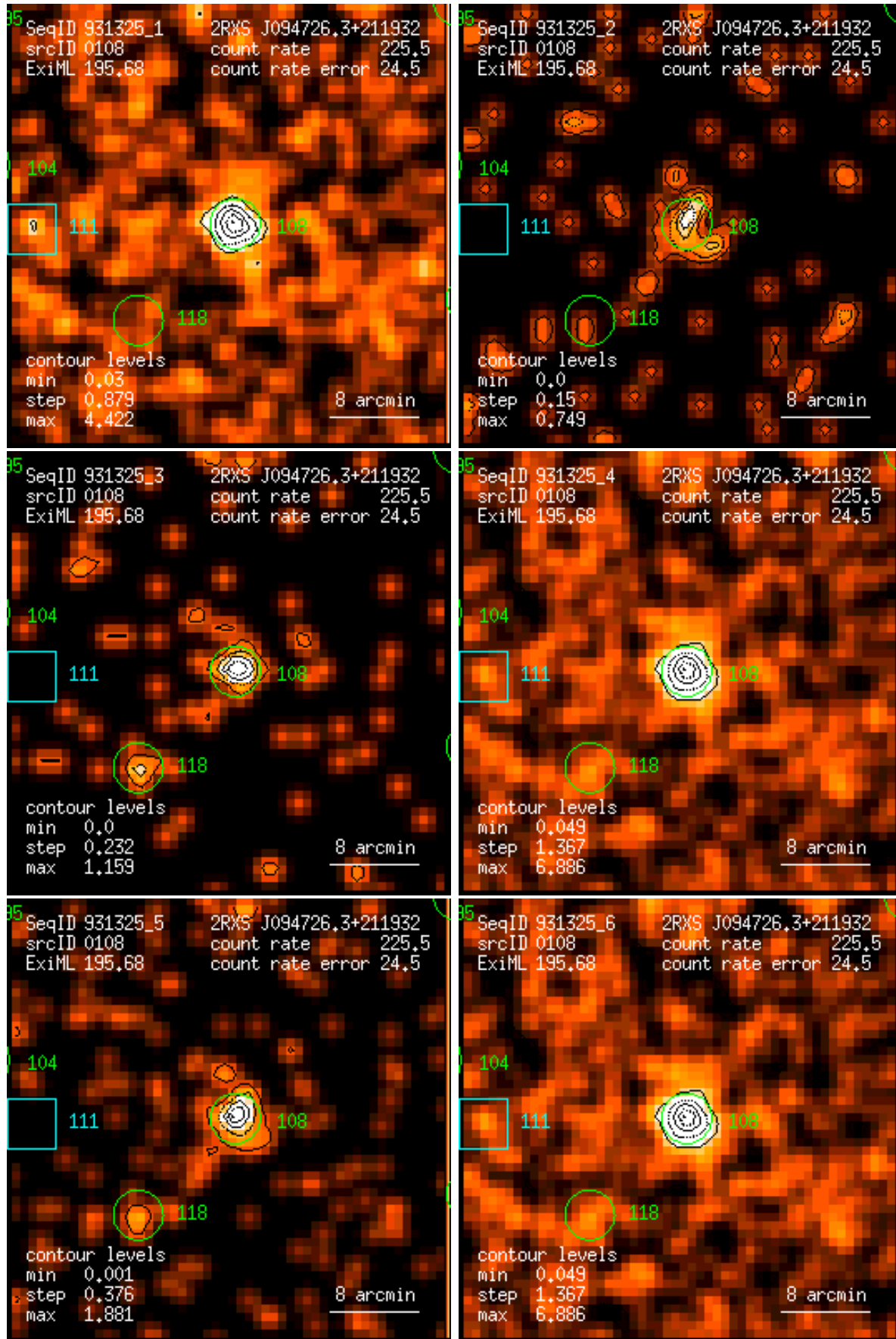
Figure 108: RASS 931325: detection 0108: band rate images, Gaussian filter: (1) PSPC channels 11 – 41, (2) 52 – 90, (3) 91 – 201, (4) 11 – 235, (5) 52 – 201, (6) 11 – 201. Broad band rates in counts/ks. Band rate contour levels in counts/ks/arcmin 2 .
