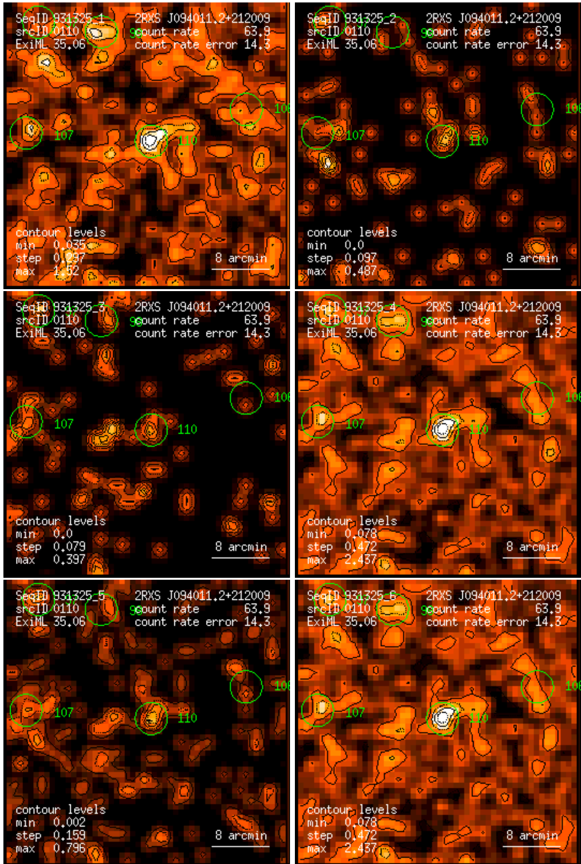
Figure 110: RASS 931325: detection 0110: band rate images, Gaussian filter: (1) PSPC channels 11 – 41, (2) 52 – 90, (3) 91 – 201, (4) 11 – 235, (5) 52 – 201, (6) 11 – 201. Broad band rates in counts/ks. Band rate contour levels in counts/ks/arcmin 2 .
