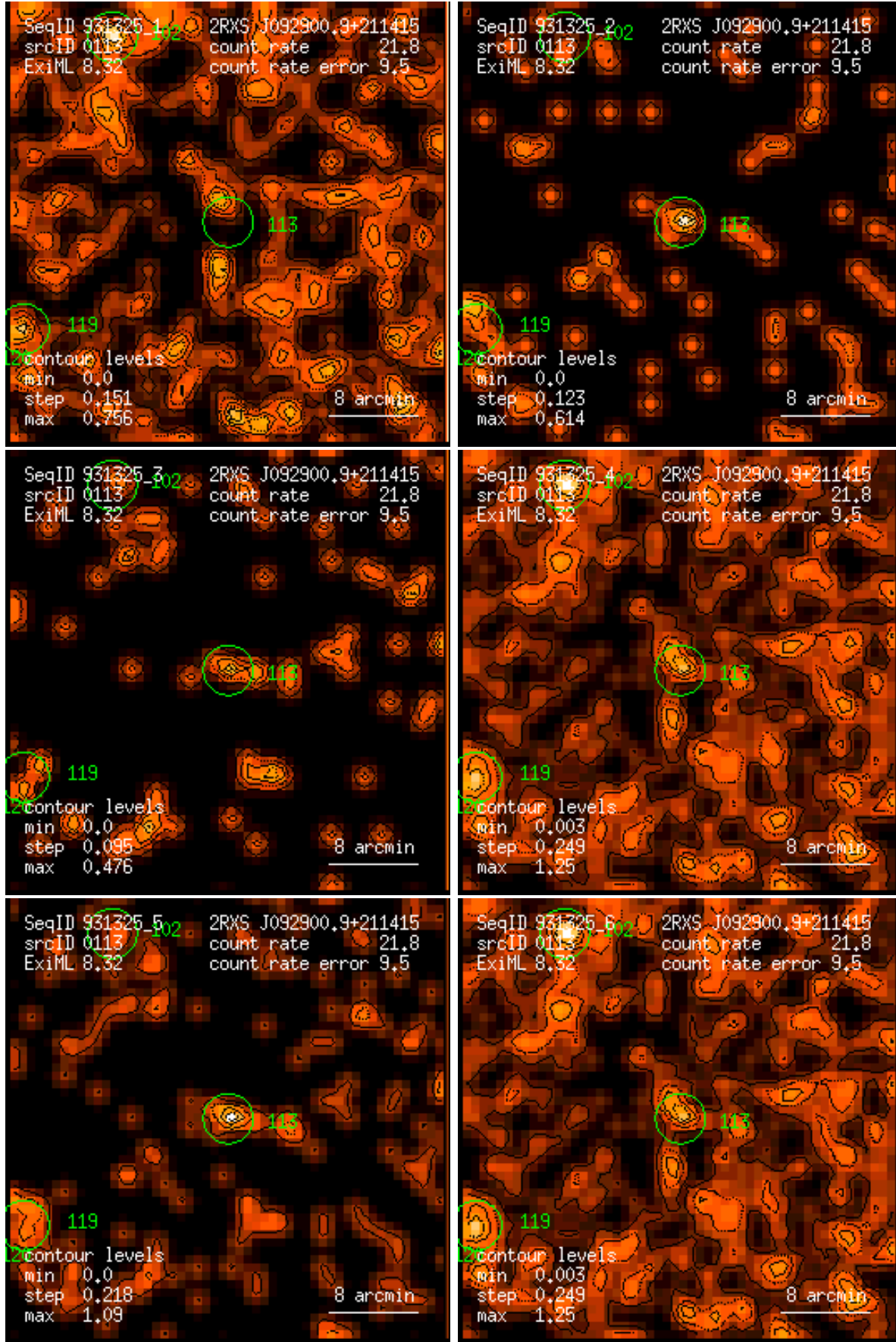
Figure 113: RASS 931325: detection 0113: band rate images, Gaussian filter: (1) PSPC channels 11 – 41, (2) 52 – 90, (3) 91 – 201, (4) 11 – 235, (5) 52 – 201, (6) 11 – 201. Broad band rates in counts/ks. Band rate contour levels in counts/ks/arcmin 2 .
