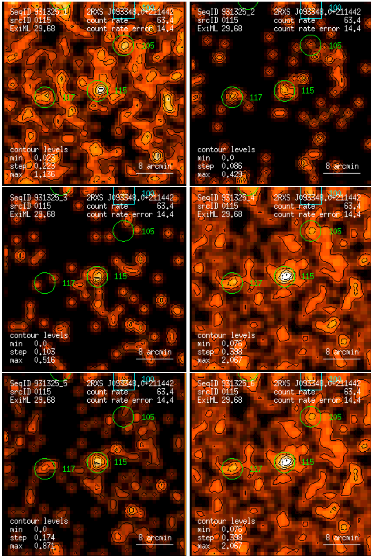
Figure 115: RASS 931325: detection 0115: band rate images, Gaussian filter: (1) PSPC channels 11 – 41, (2) 52 – 90, (3) 91 – 201, (4) 11 – 235, (5) 52 – 201, (6) 11 – 201. Broad band rates in counts/ks. Band rate contour levels in counts/ks/arcmin 2 .
