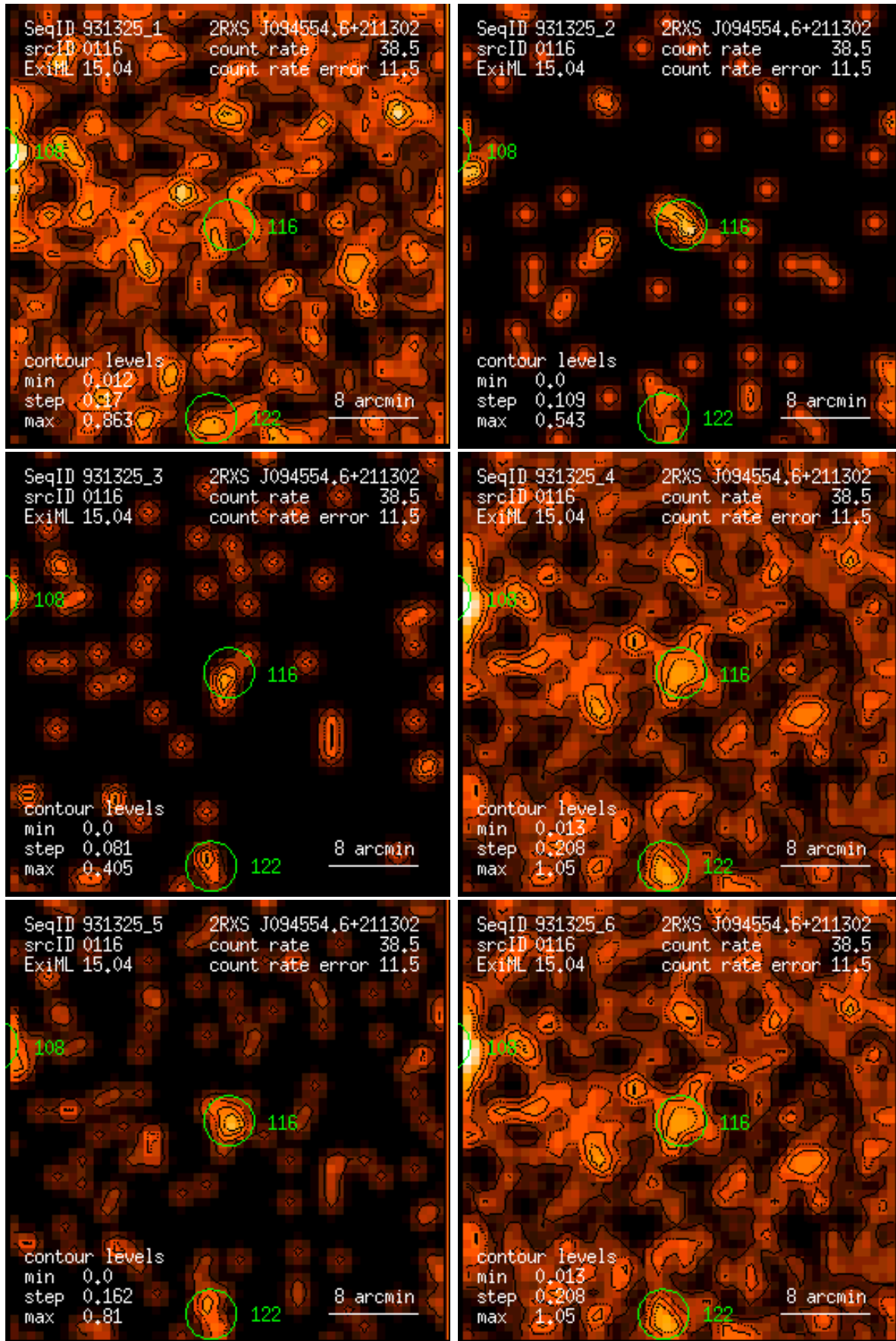
Figure 116: RASS 931325: detection 0116: band rate images, Gaussian filter: (1) PSPC channels 11 – 41, (2) 52 – 90, (3) 91 – 201, (4) 11 – 235, (5) 52 – 201, (6) 11 – 201. Broad band rates in counts/ks. Band rate contour levels in counts/ks/arcmin 2 .
