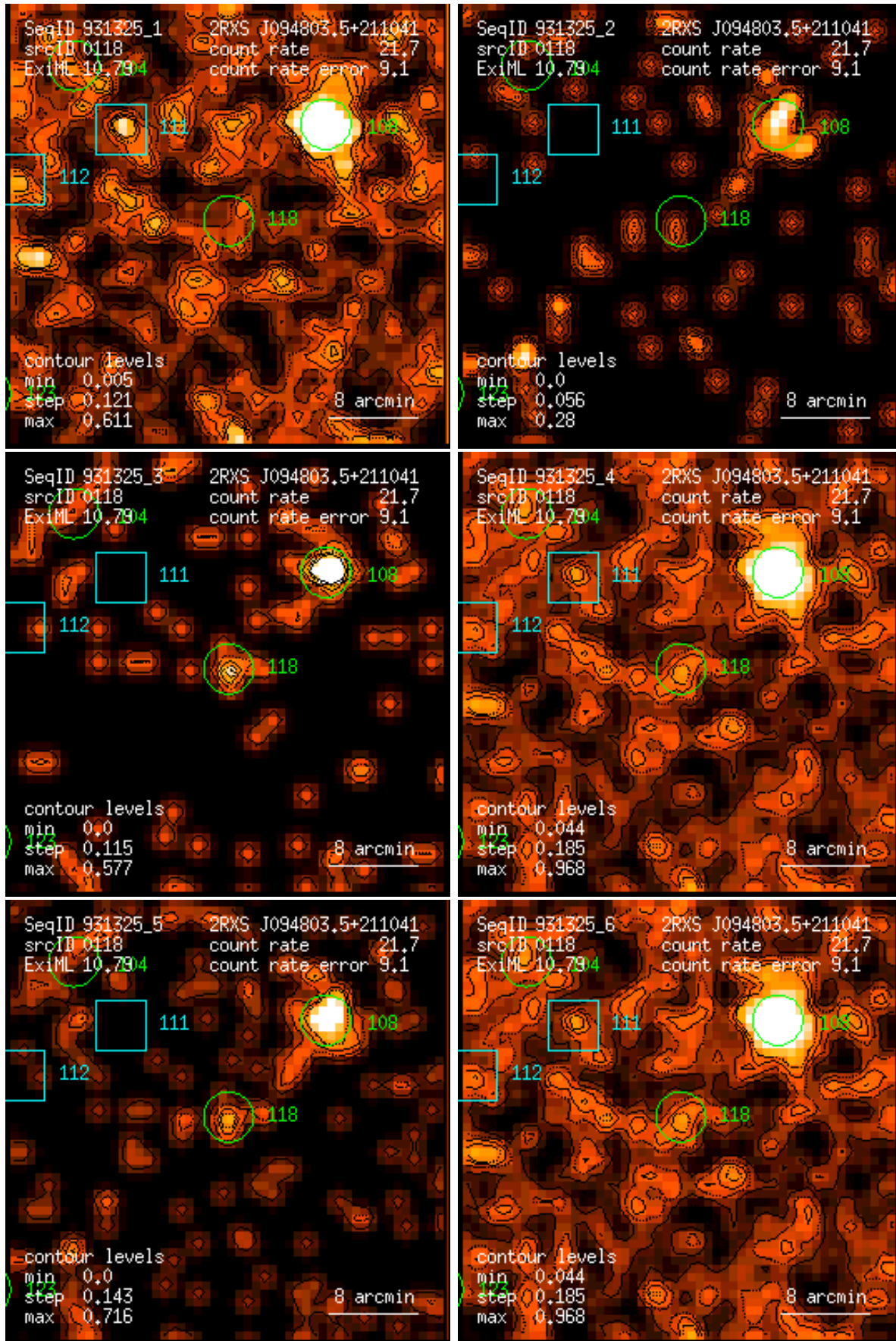
Figure 118: RASS 931325: detection 0118: band rate images, Gaussian filter: (1) PSPC channels 11 – 41, (2) 52 – 90, (3) 91 – 201, (4) 11 – 235, (5) 52 – 201, (6) 11 – 201. Broad band rates in counts/ks. Band rate contour levels in counts/ks/arcmin 2 .
