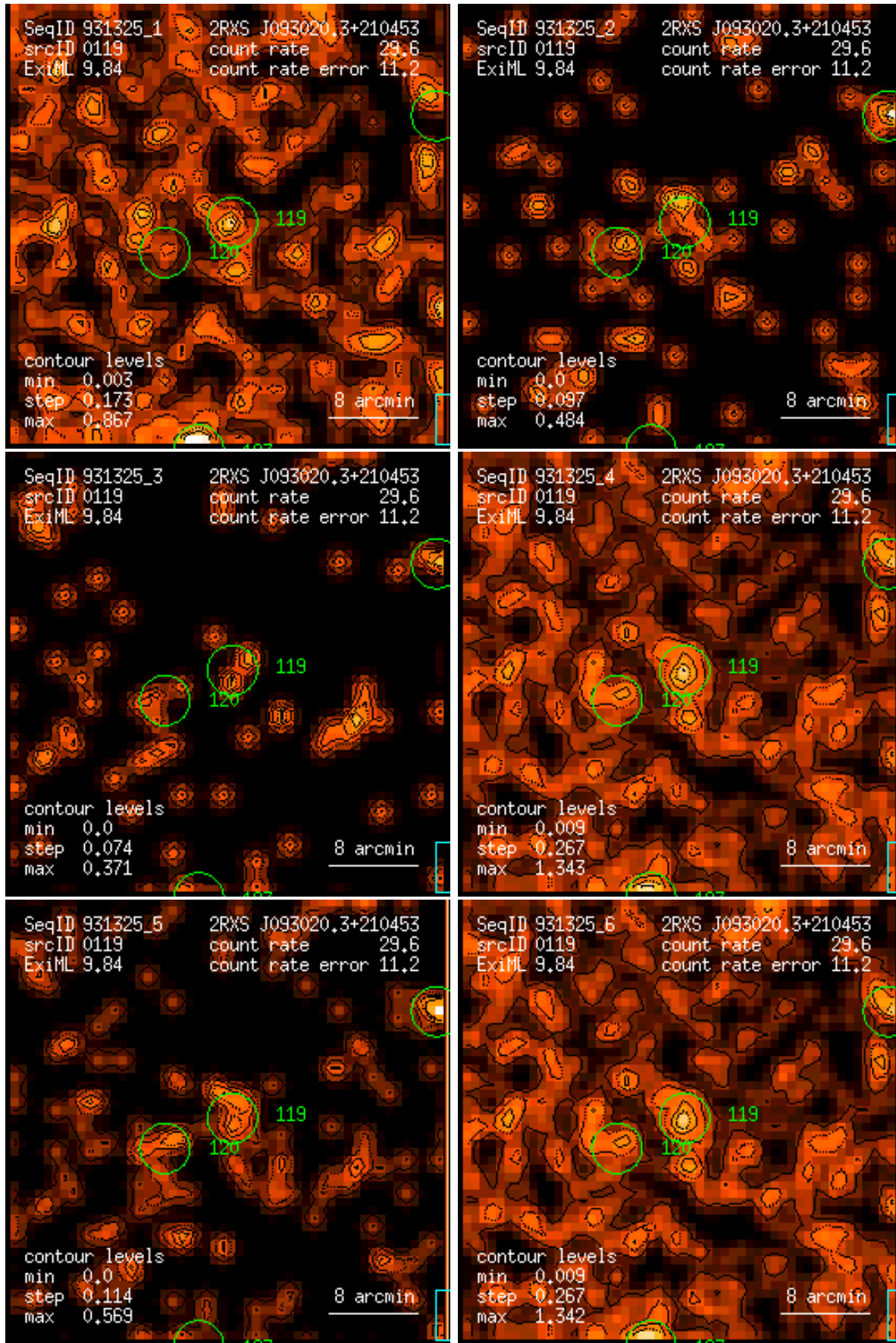
Figure 119: RASS 931325: detection 0119: band rate images, Gaussian filter: (1) PSPC channels 11 – 41, (2) 52 – 90, (3) 91 – 201, (4) 11 – 235, (5) 52 – 201, (6) 11 – 201. Broad band rates in counts/ks. Band rate contour levels in counts/ks/arcmin 2 .
