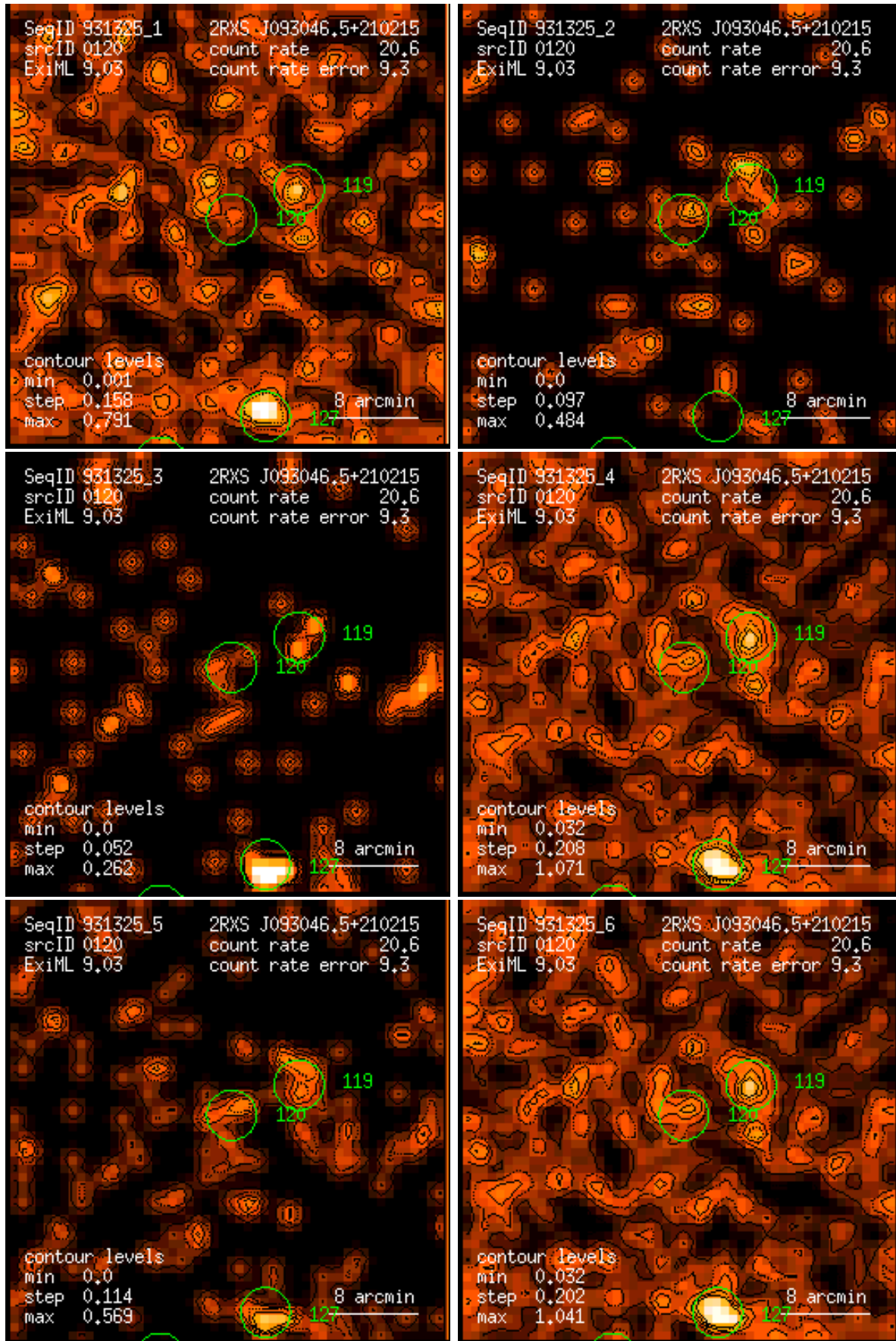
Figure 120: RASS 931325: detection 0120: band rate images, Gaussian filter: (1) PSPC channels 11 – 41, (2) 52 – 90, (3) 91 – 201, (4) 11 – 235, (5) 52 – 201, (6) 11 – 201. Broad band rates in counts/ks. Band rate contour levels in counts/ks/arcmin 2 .
